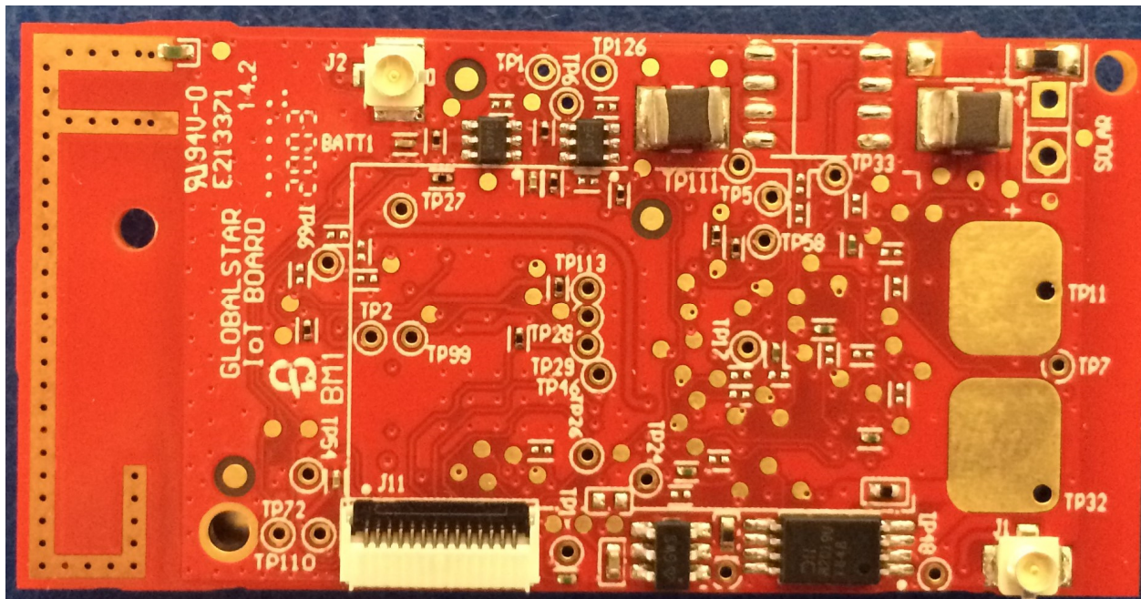
Picture 1: Battery Side of ST100
