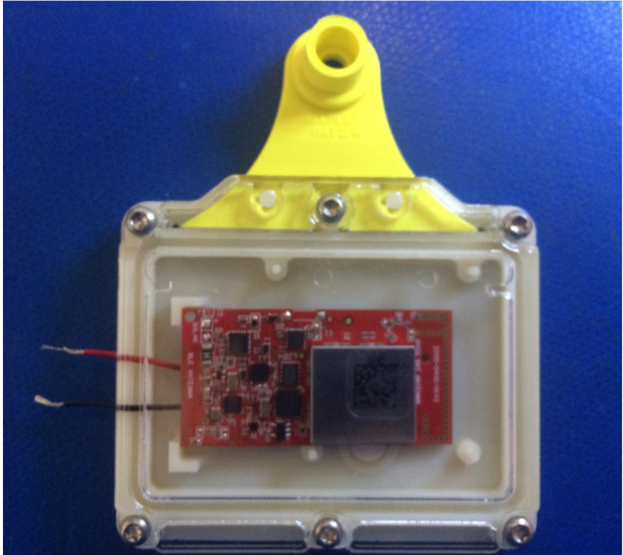
Picture 3 - ST100 module installed in ST100 Basic (Host) – Front
