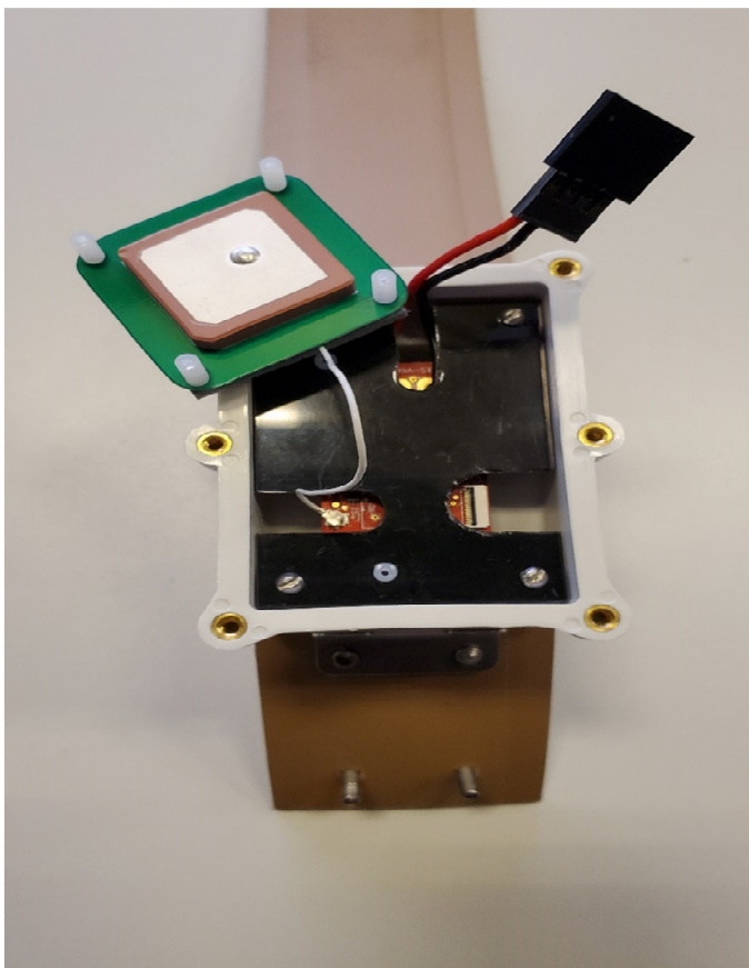
Better Look at the External Antenna
