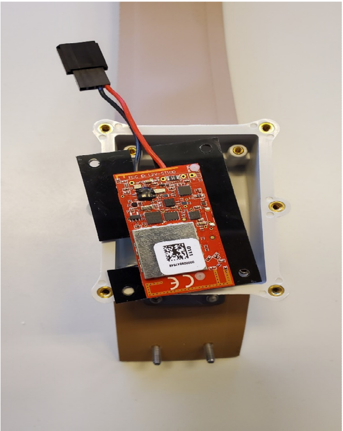
Better Look at the Electronics Assemblie – Internal Antenna
