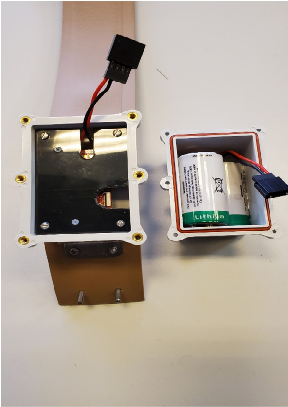
Housing Opened Up Bottom View – Internal Antenna
