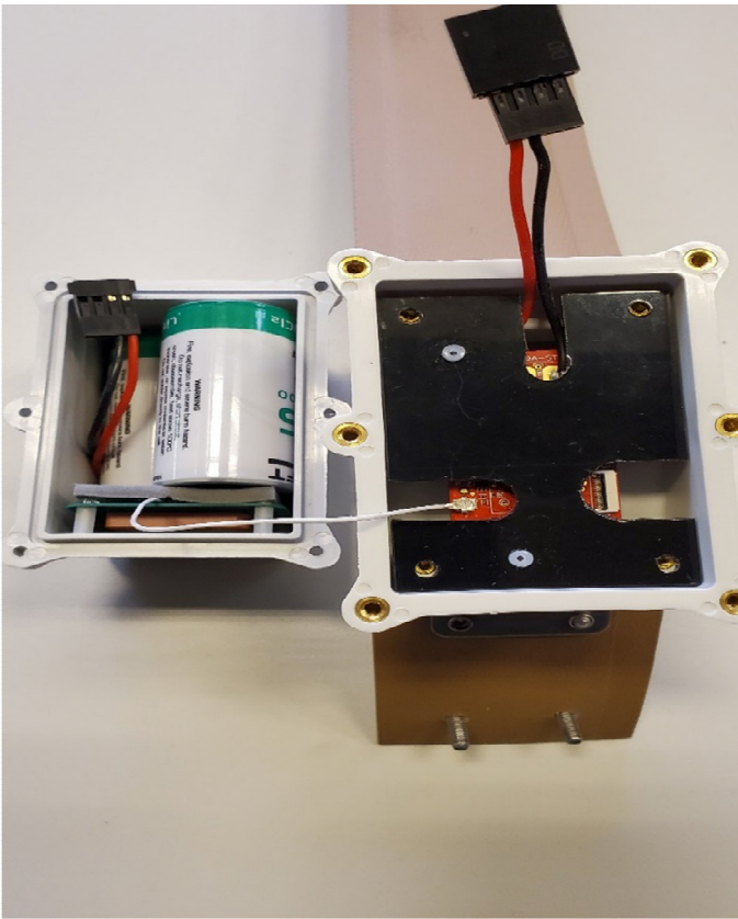
Housing Opened up – External Antenna
