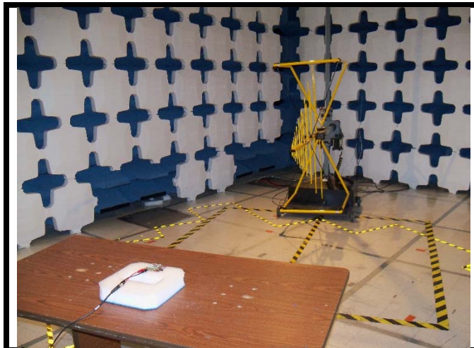
Test Setup Photo # 4
