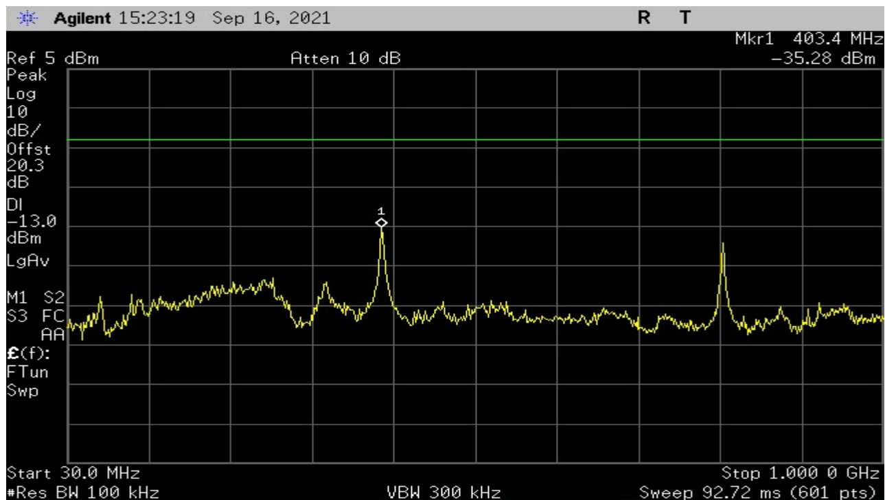
Plot 13 Highest Channel – 30MHz to 1GHz
