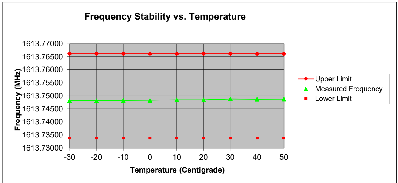
Plot 27 – Temperature vs Frequency
