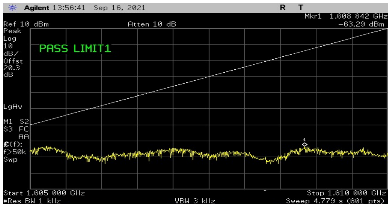
Plot 22-High Channel – Test Limit 25.216 (f)(g) – Discrete Emissions
