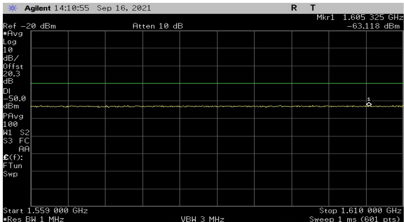
Plot 26 – High Channel – Carrier Off
