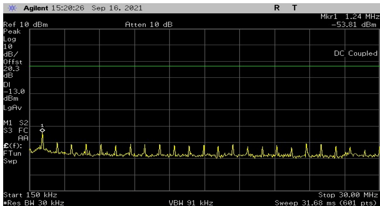
Plot 7 – Lowest Channel - 150kHz to 30MHz
