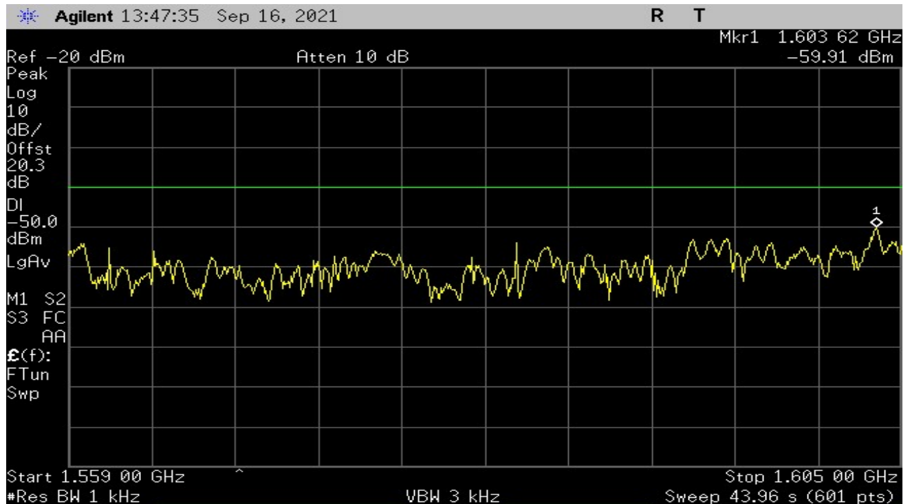
Plot 17 – Low Channel – Test Limit 25.216 (c) – Discrete Emissions
