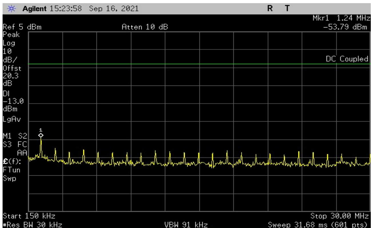
Plot 12 – Highest Channel – 150kHz to 30MHz
