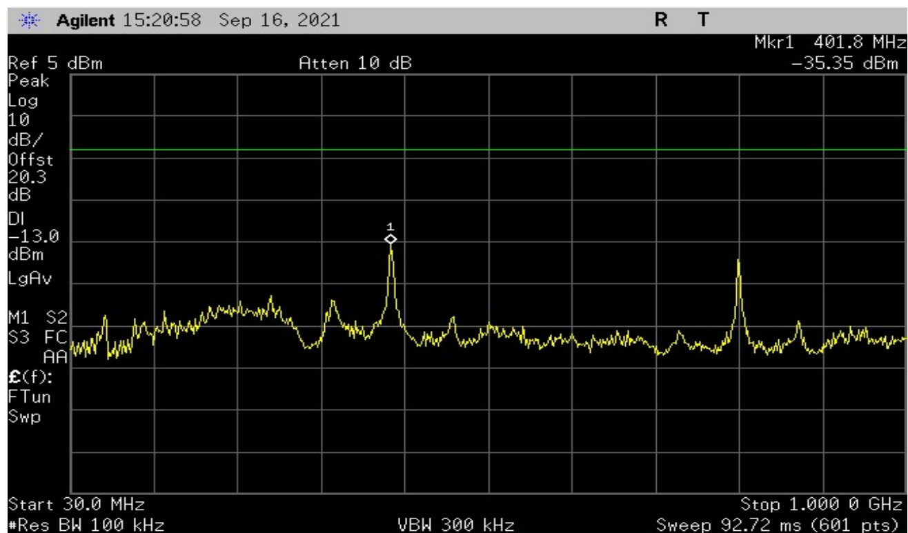
Plot 8 – Lowest Channel - 30MHz to 1GHz
