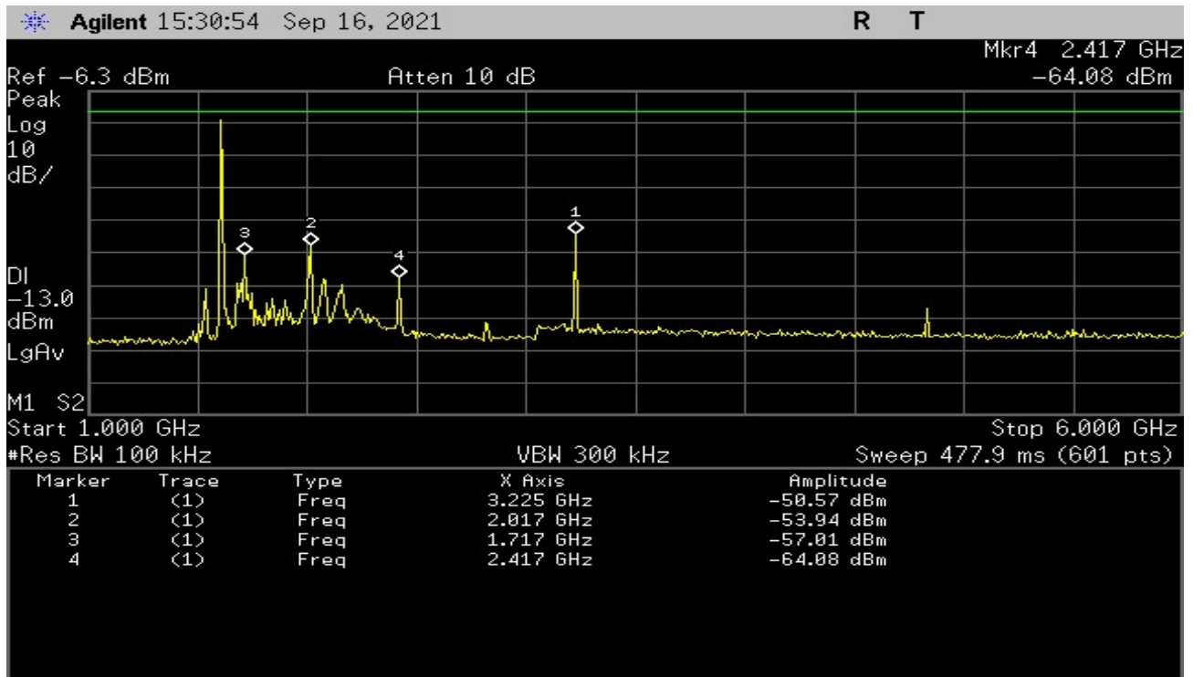
Plot 9 – Lowest Channel - 1GHz to 6GHz
