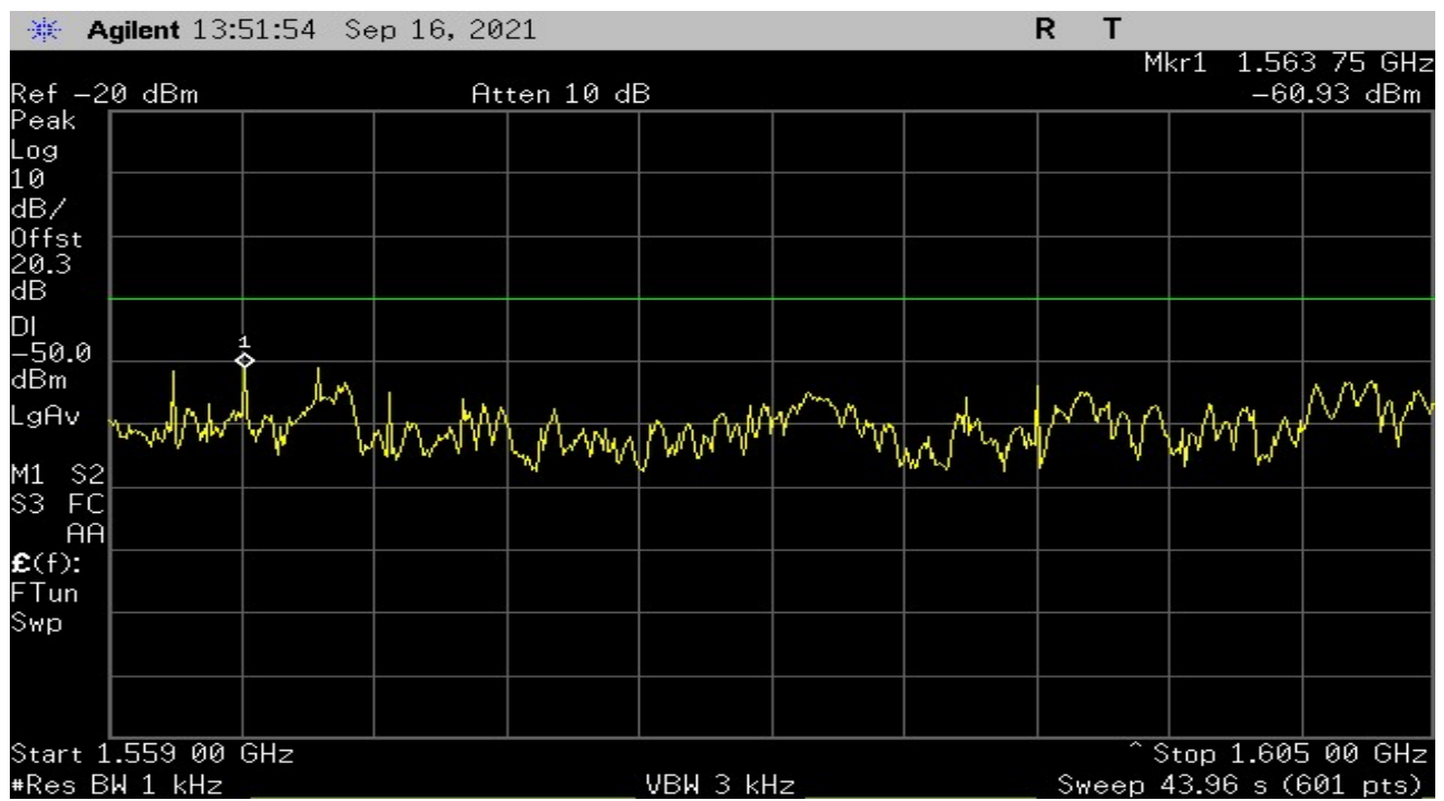
Plot 18 – High Channel – Test Limit 25.216 (c) – Discrete Emissions
