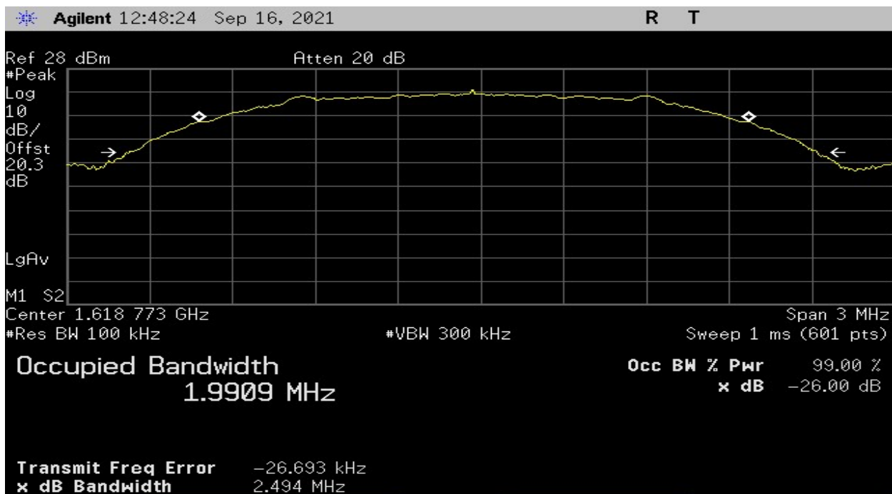
Plot 4 – High Channel – 26dB Bandwidth
