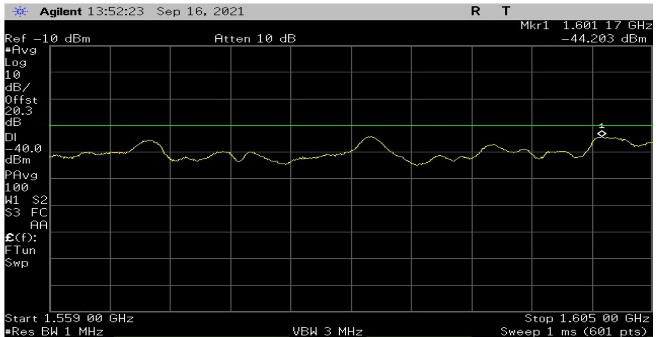
Plot 20 – High Channel – Test Limit 25.216 (c)
