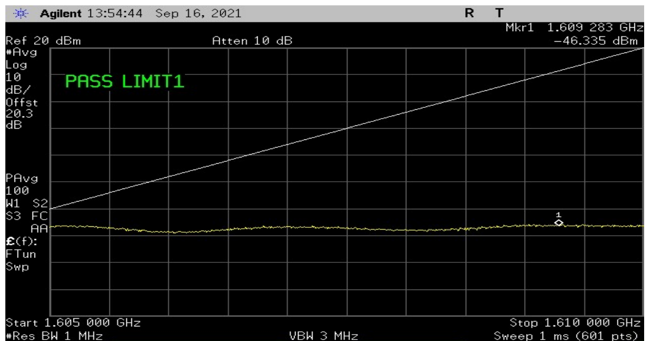
Plot 24-High Channel – Test Limit 25.216 (f)(g)
