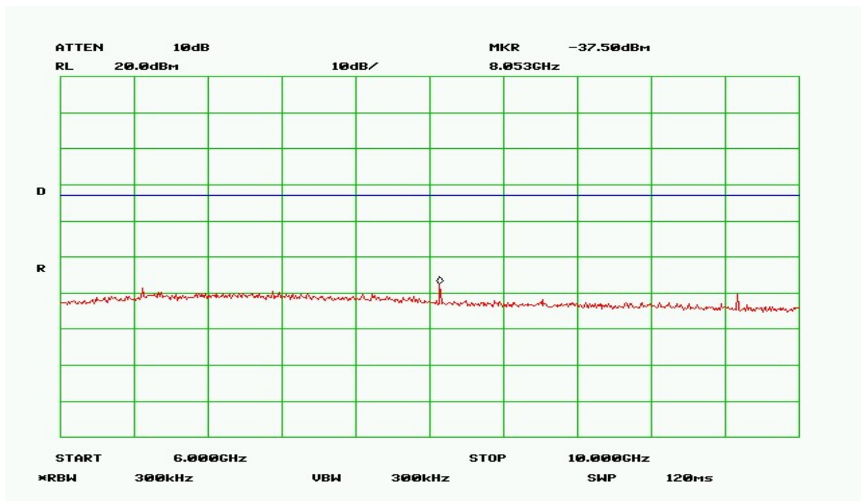
Plot 10 – Lowest Channel - 6GHz to 10 GHz
