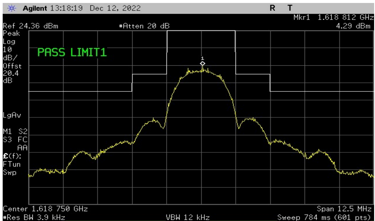
Plot 6 – Emission Mask - High Channel
