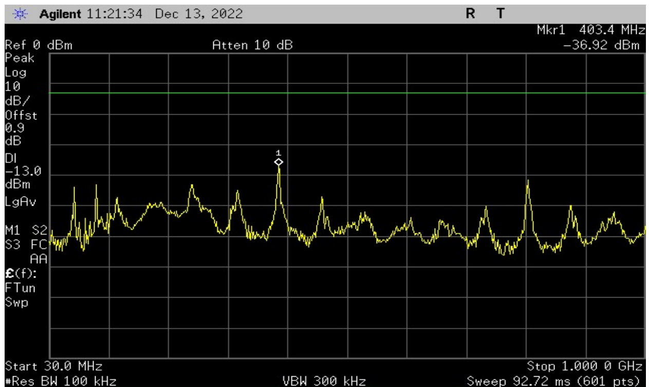
Plot 13 Highest Channel – 30MHz to 1GHz
