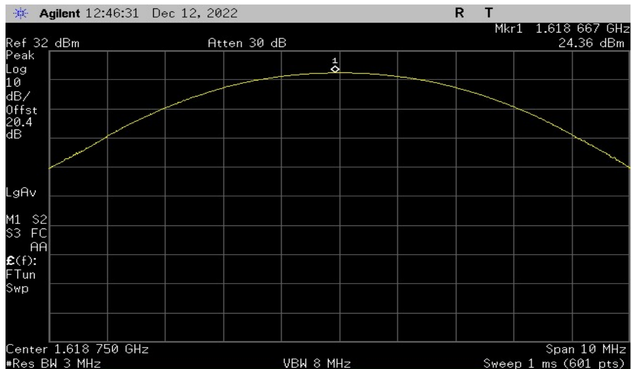
Plot 2 – Output Power – High Channel
