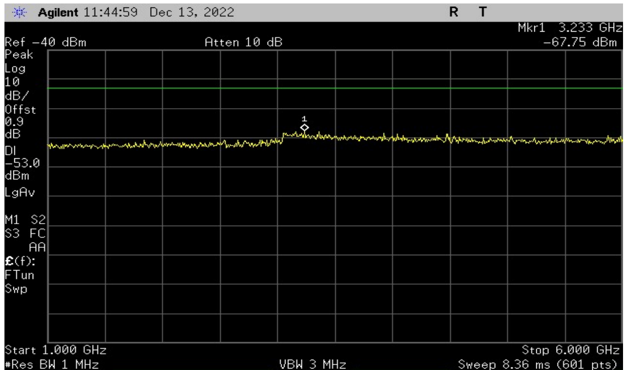
Plot 18 – Receiver Spurious Emissions – 1GHz to 6GHz (For Industry Canada)
