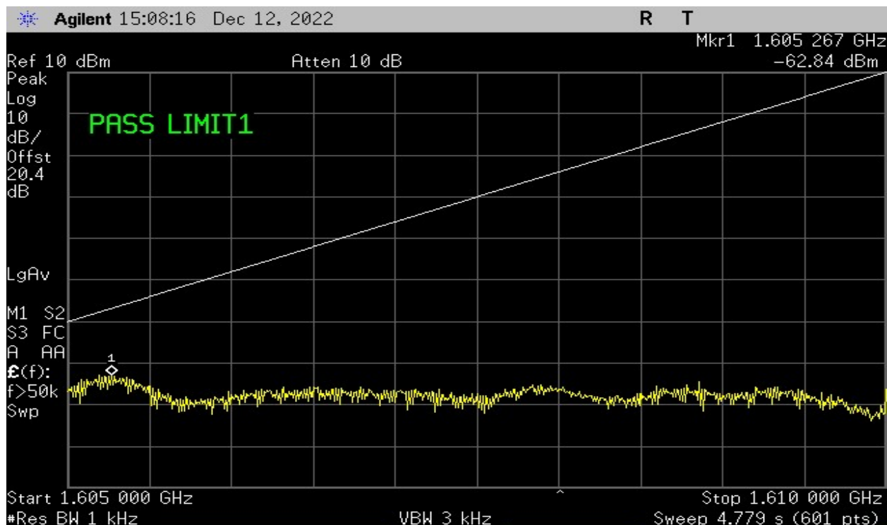
Plot 24-High Channel – Test Limit 25.216 (f)(g) – Discrete Emissions
