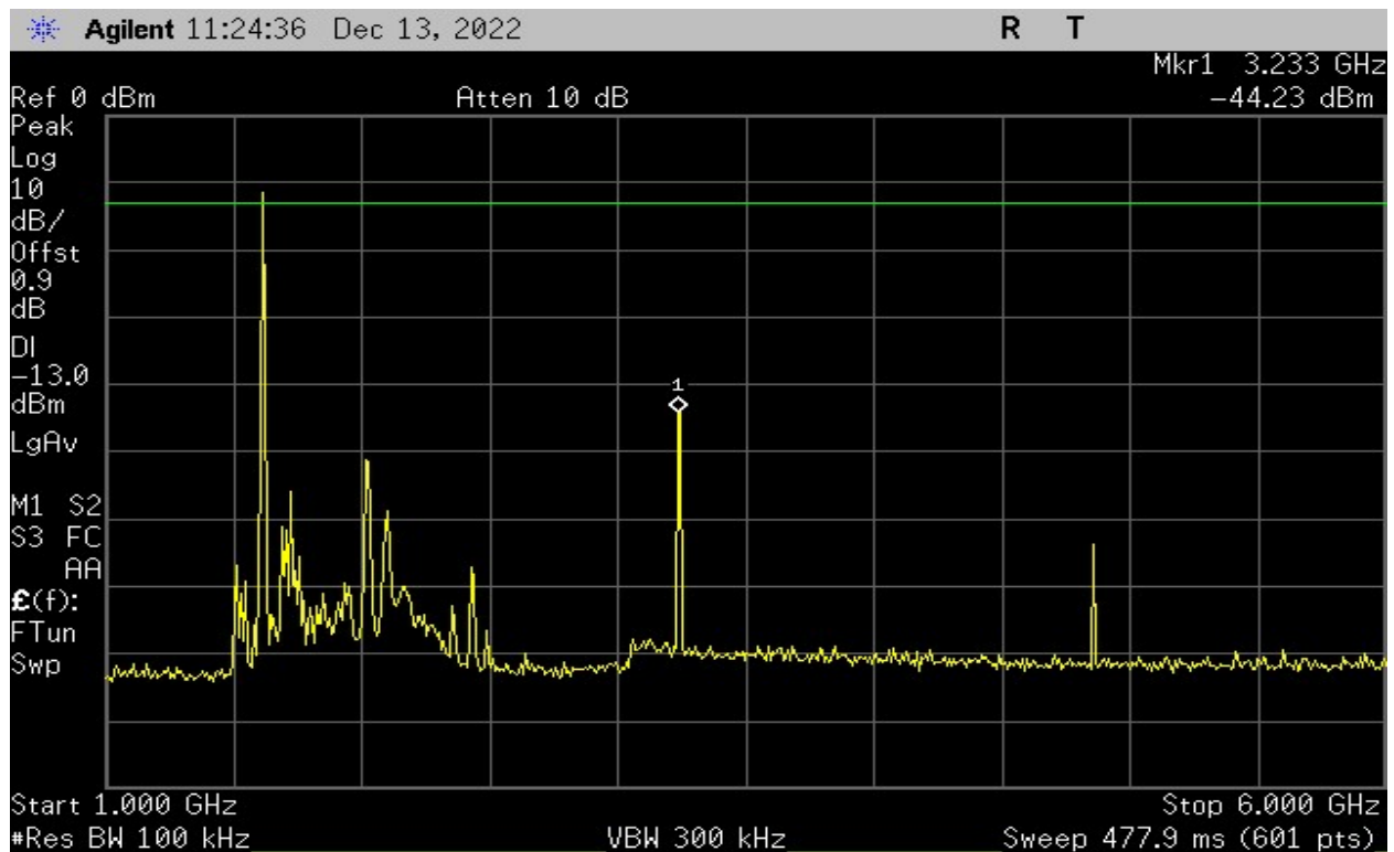
Plot 14 Highest Channel - 1GHz to 6GHz
