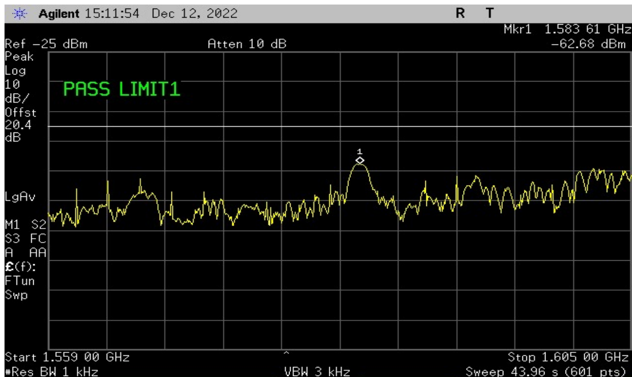
Plot 20 – High Channel – Test Limit 25.216 (c) – Discrete Emissions
