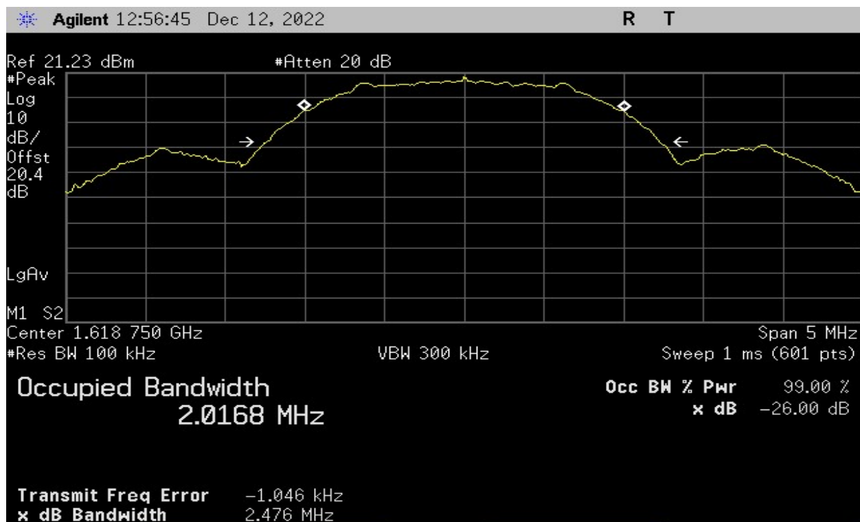
Plot 4 – High Channel – 26dB Bandwidth
