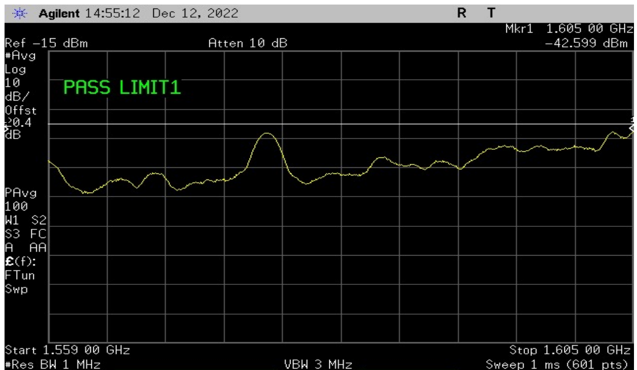
Plot 21 – Low Channel – Test Limit 25.216 (c)
