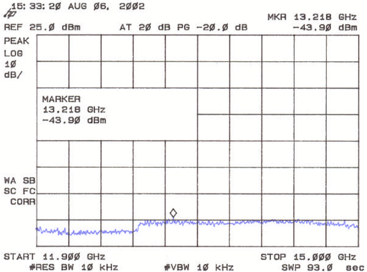
Figure 6f. Spurious Emissions at Antenna Terminals
