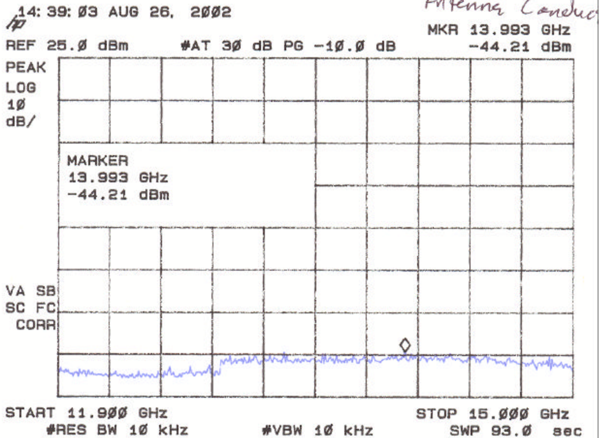
Figure 6n. Spurious Emissions at Antenna Terminals
