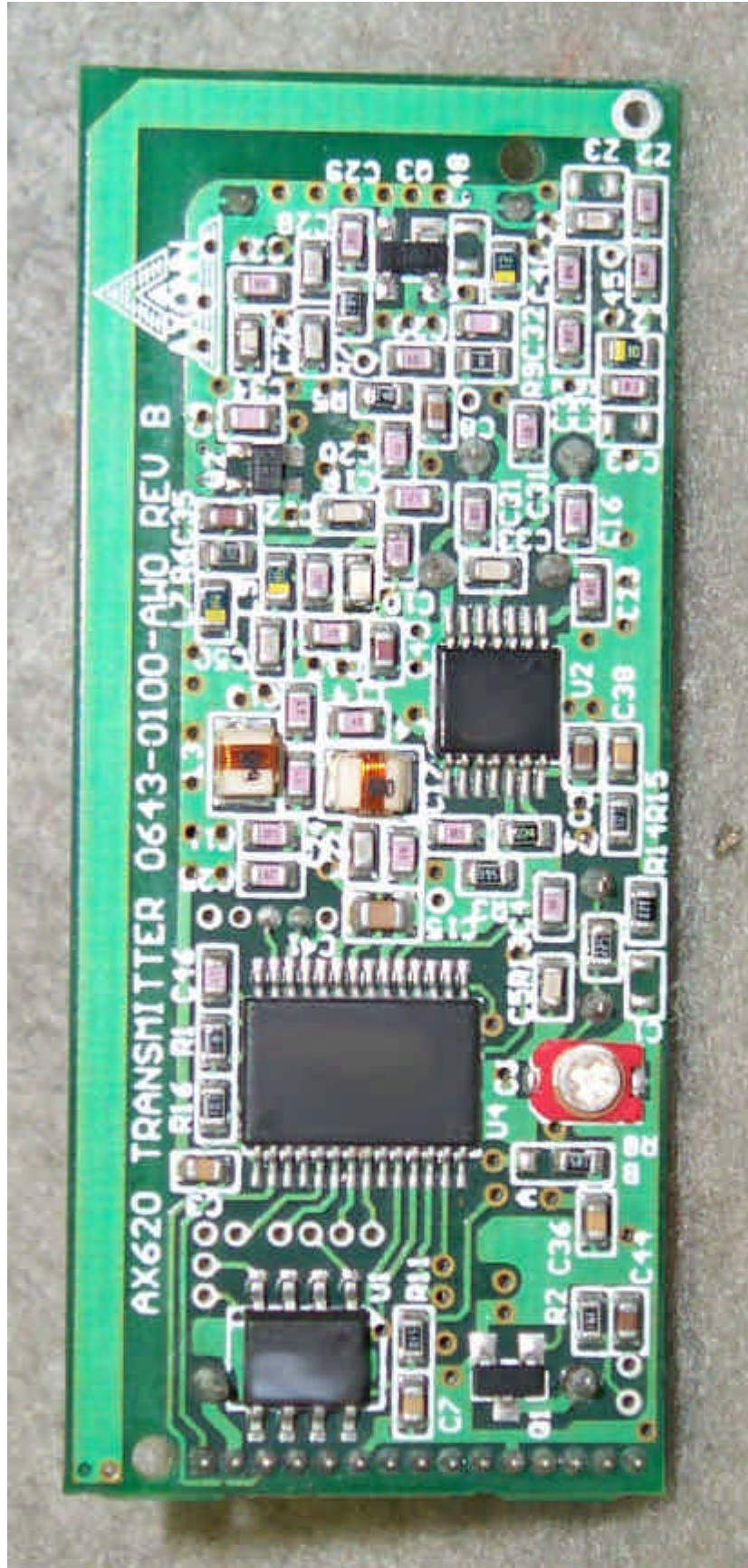
Photo 4. EUT, Top View
