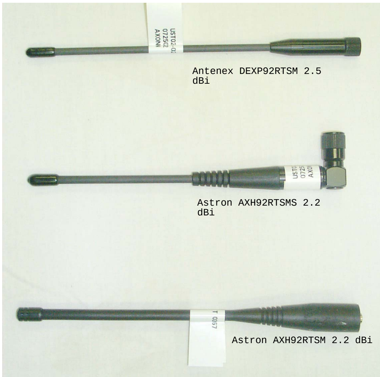
Photo 4. Antennas
