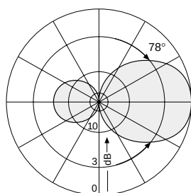
Vertical Pattern 60 mm Ø
