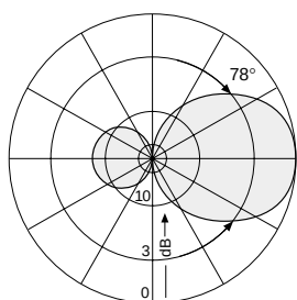
Vertical Pattern 115 mm Ø
