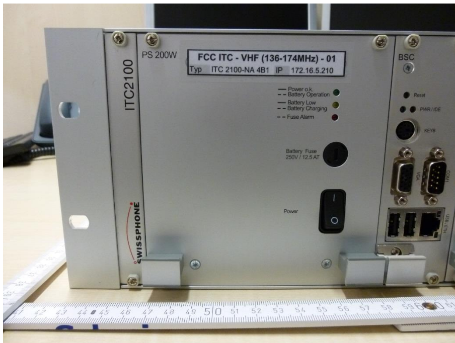
Photo 2: Front detailed
