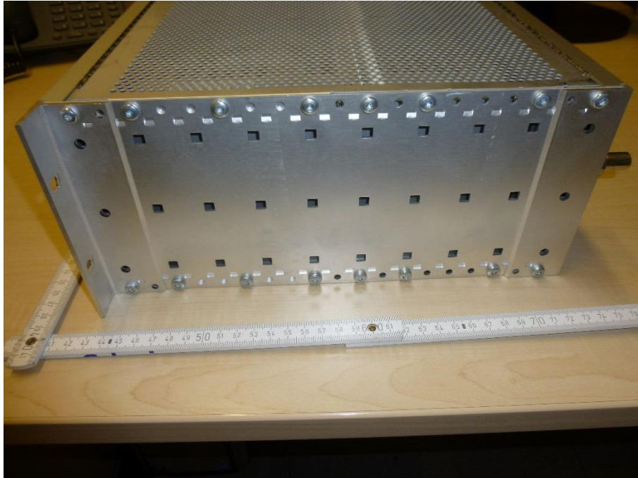
Photo 5: Right side
