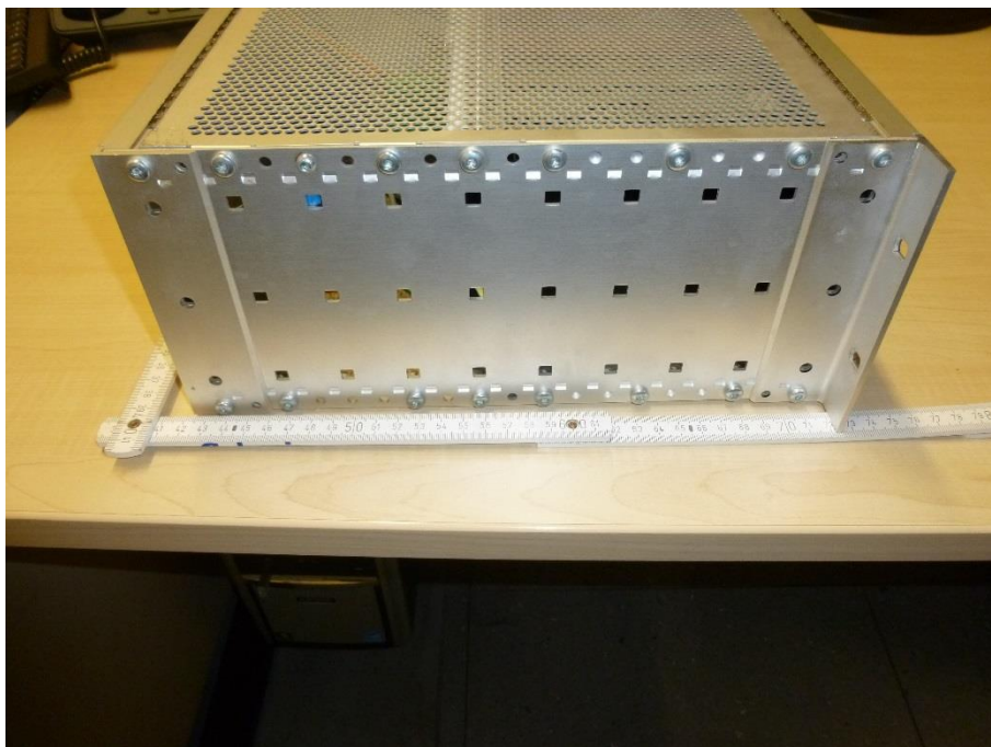
Photo 6: Left side
