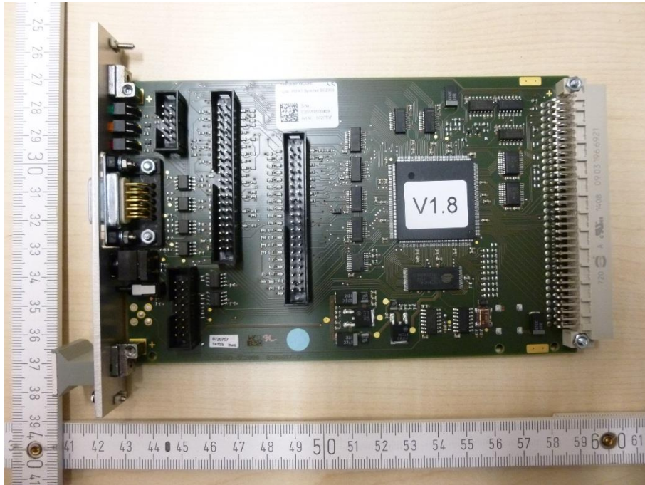
Photo 25: SC module
