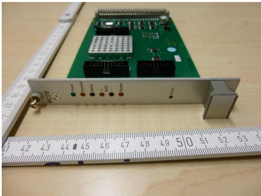
Photo 20: RC09 module
