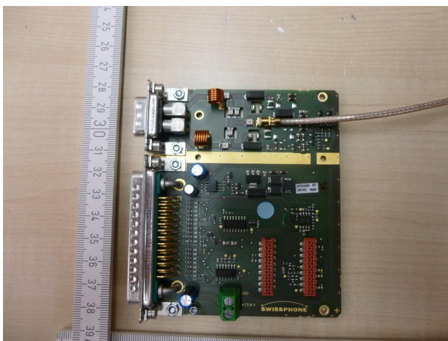
Photo 48: RF module
