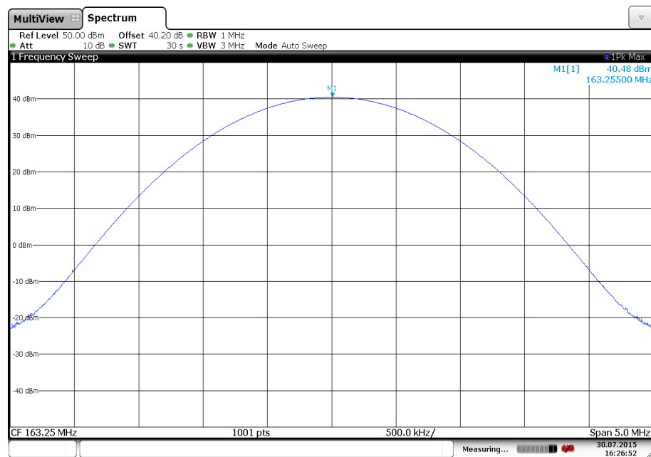
Plot 2: Middle channel – Low power
