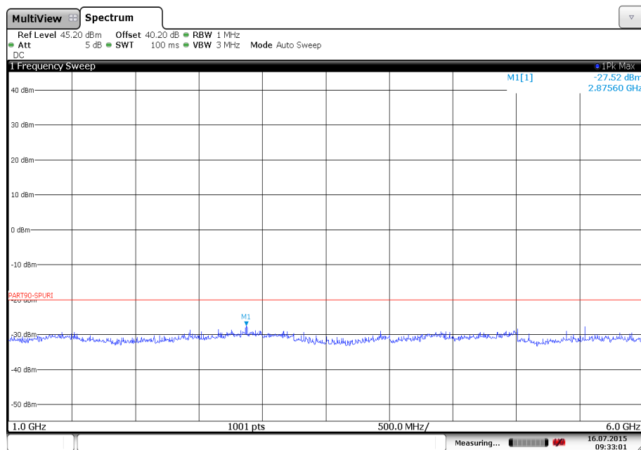
Plot 8: Low channel – High power – 1 GHz to 6 GHz
