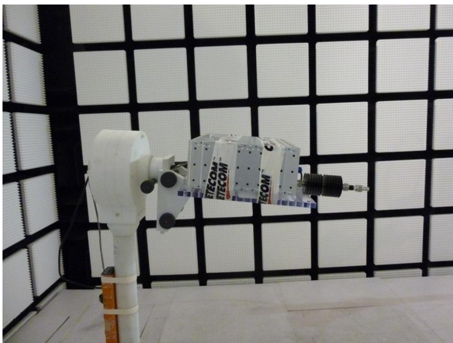
Photo 2: Measurements fully anechoic chamber
