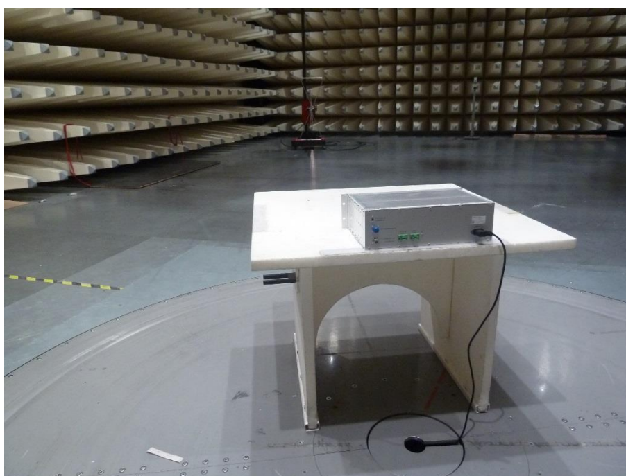
Photo 8: Measurements semi anechoic chamber
