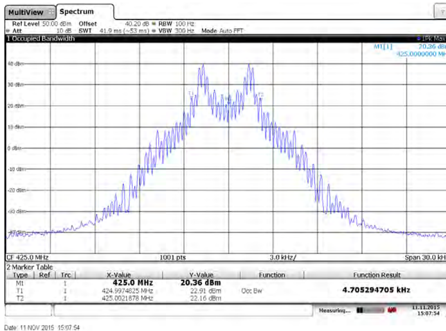
Plot 2: Middle channel / 512 bits per second
