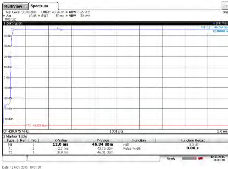
Plot 10: Highest channel – Switch on (zoomed)
