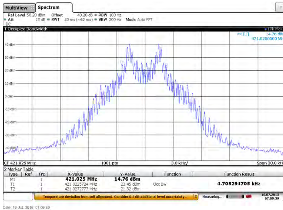
Plot 1: Low channel / 512 bits per second
