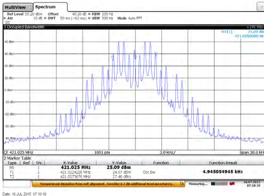
Plot 4: Low channel / 1200 bits per second
