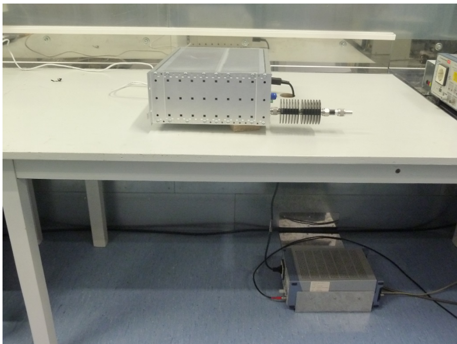
Photo 6: AC-conducted measurements
