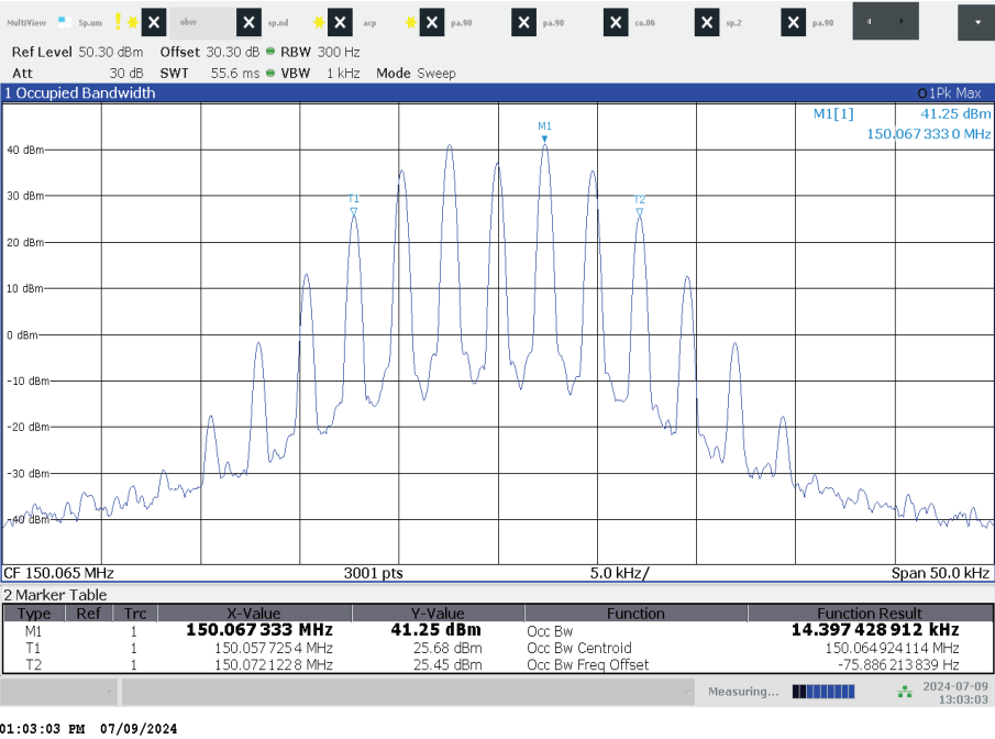
Plot 4: low channel / 4800 bits per second
