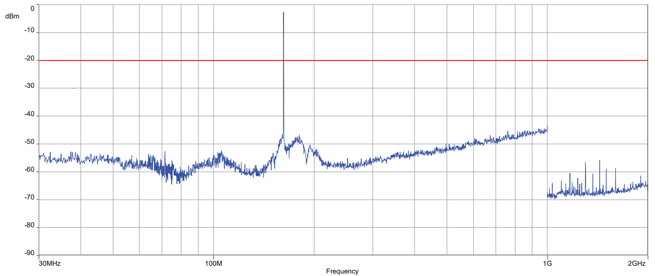
Plot 2: 30 MHz – 2 GHz, middle channel, antenna vertical/horizontal
