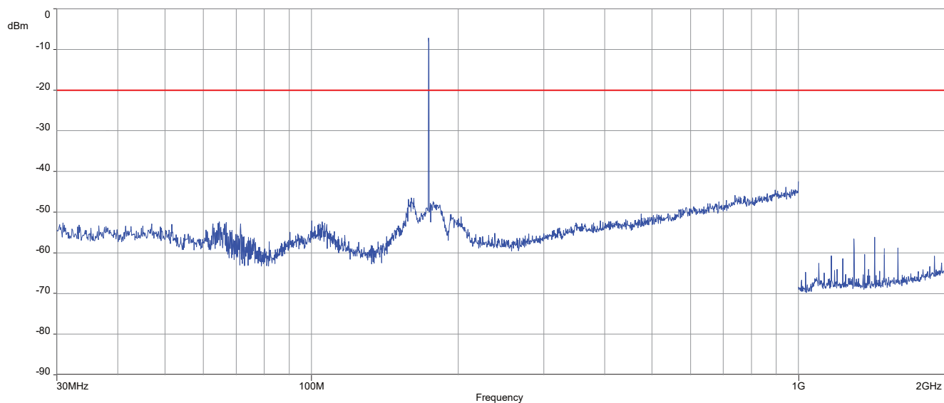
Plot 3: 30 MHz – 2 GHz, high channel, antenna vertical/horizontal
