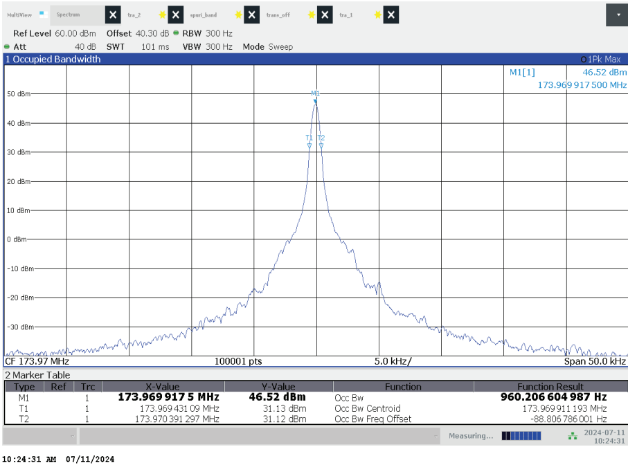
Plot 9: high channel – carrier
