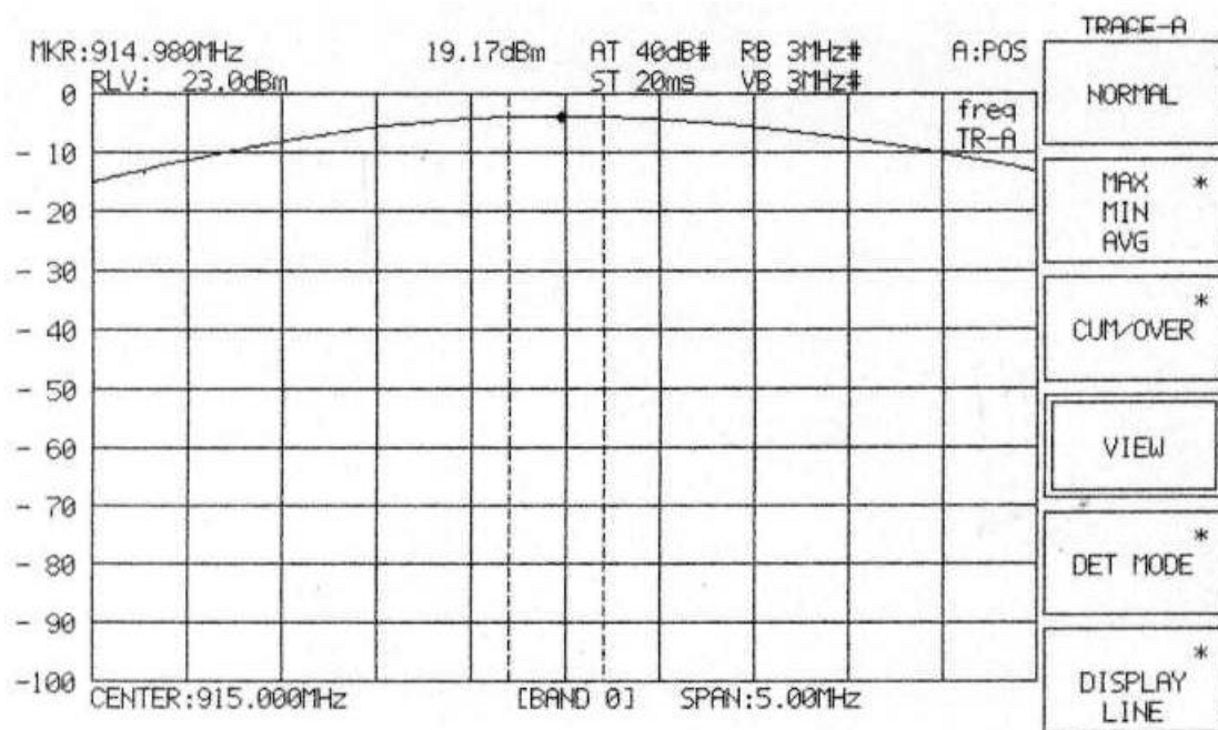
Maximum Power Output 915MHz
