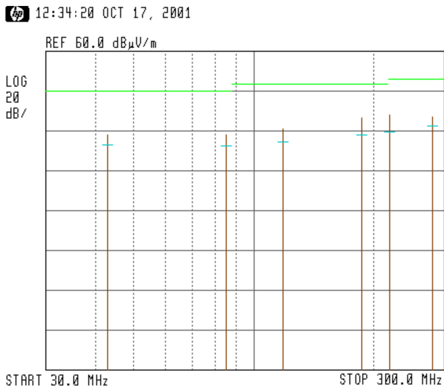
Figure 52. Radiated Emission. Antenna Polarization: VERTICAL. Detectors: Peak, Quasi-peak
