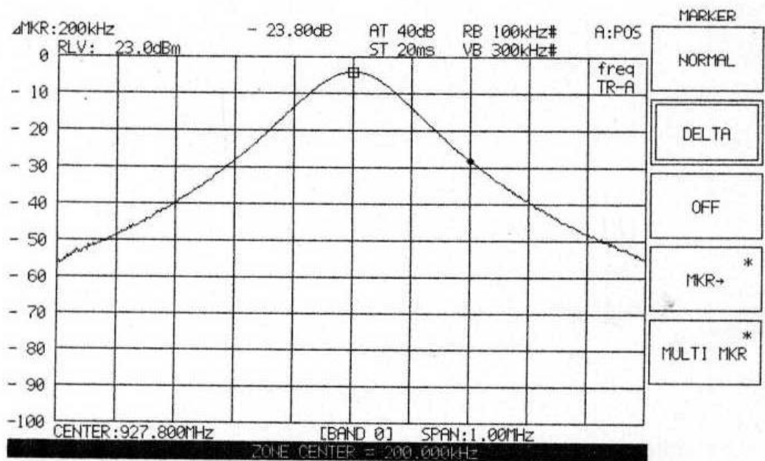
Band Edge Spectrum of 927.8MHz
