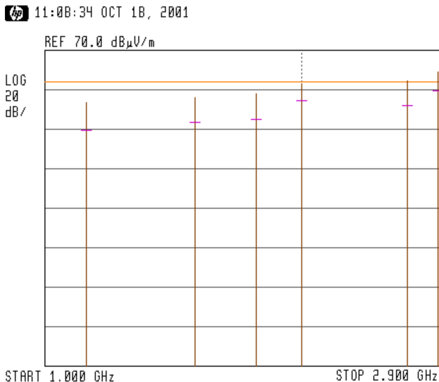
Figure 57. Radiated Emission. Antenna Polarization: VERTICAL Detectors: Peak, Average
