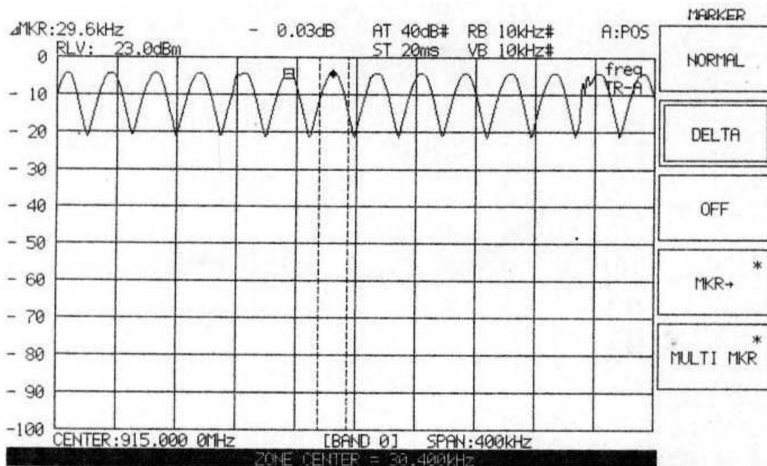
Hopping Channels Separation In 915 MHz Figure 81
