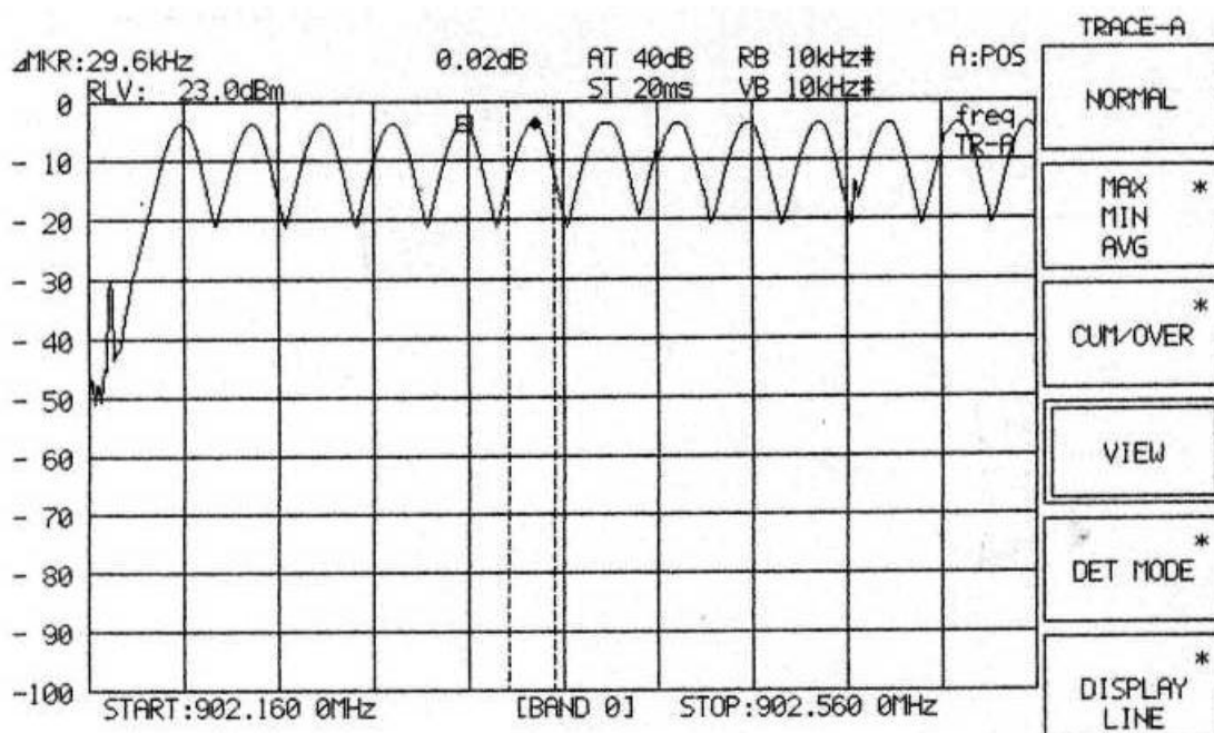
Hopping Channels Separation In 902.2 MHz Figure 80
