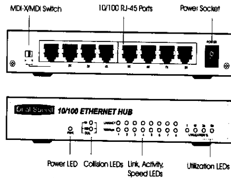
Figure 1-1 Front & Back view of the Hub
