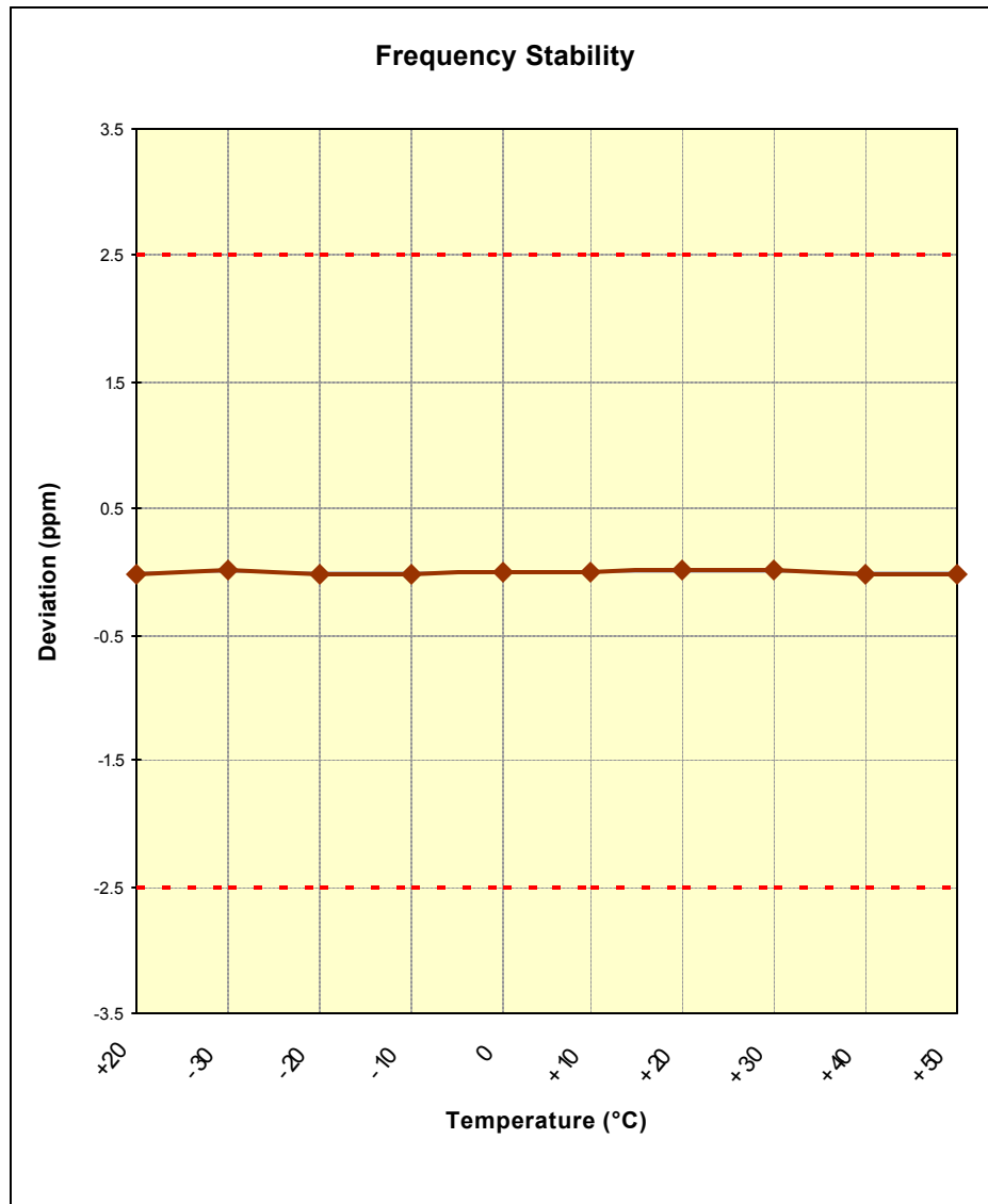
Figure 6-2. Frequency Stability Graph (Cellular CDMA Mode – Ch. 384)
