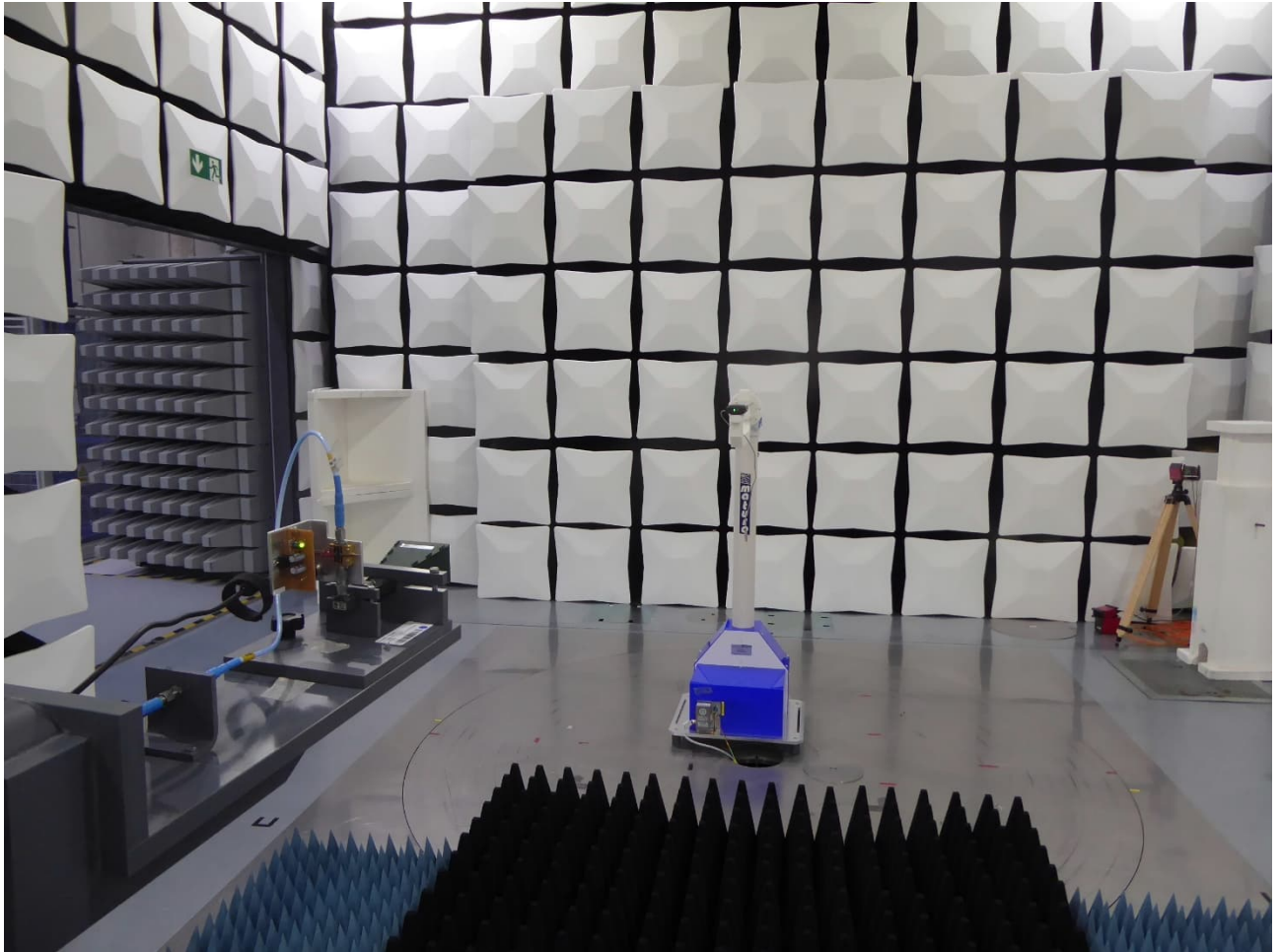
Test Setup 18 GHz - 26.5 GHz
