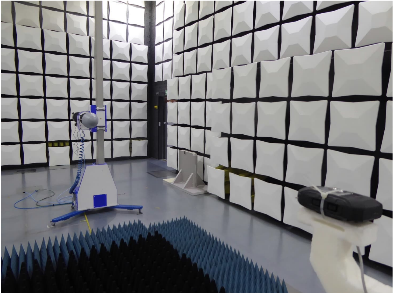
Test Setup 12 GHz – 18 GHz
