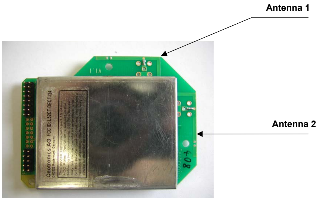
Photo 1 : Antenna Position
