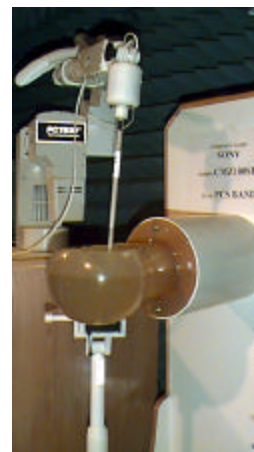
Figure 1. SAR Test Set-up
