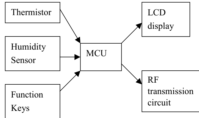
0781-H Tx block diagram
