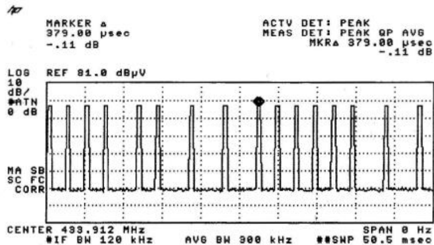
Figure C [Short Pulse]
