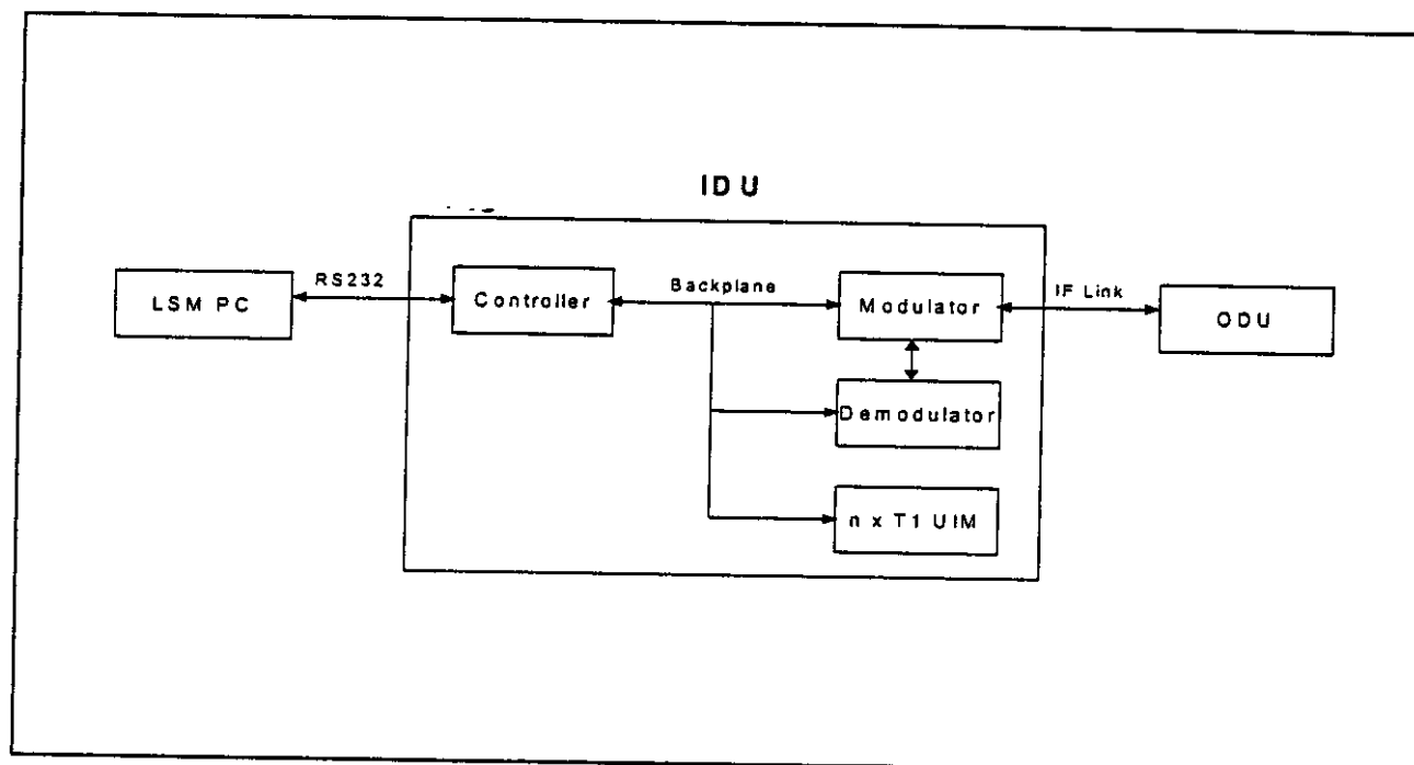
Figure 4-3 – IDU Block Diagram
