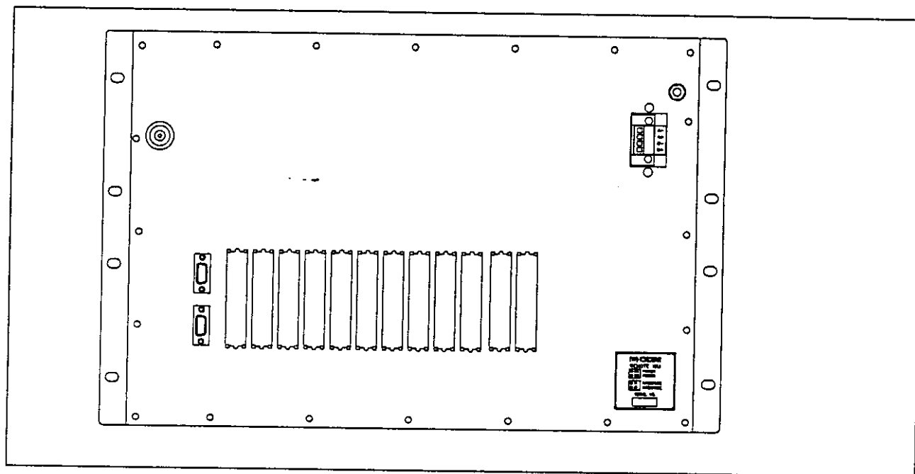
Figure 4-7 - Remote Terminal Rear View (DC Input Power)
