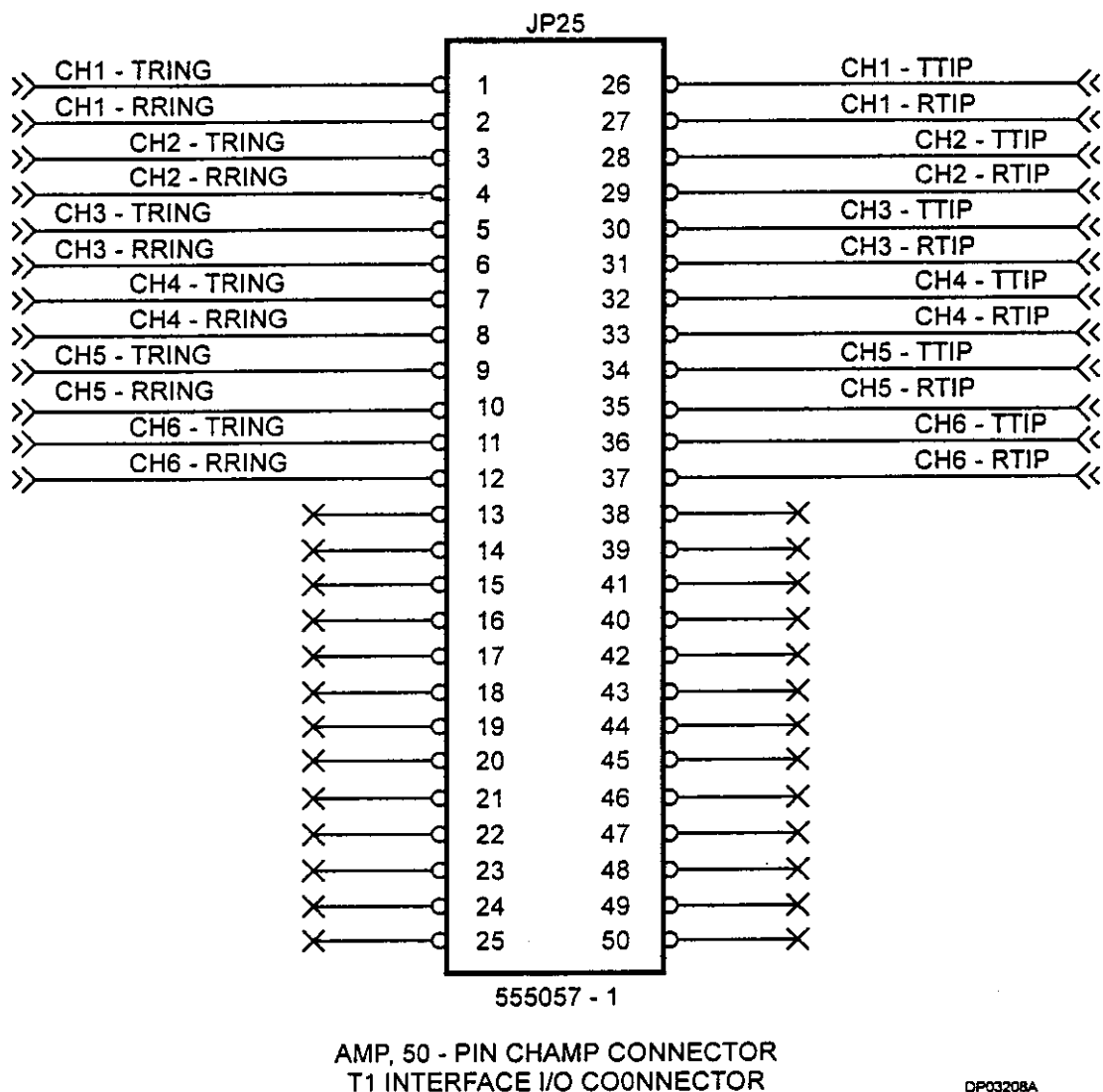
Figure 8-5 - NIC pinouts
