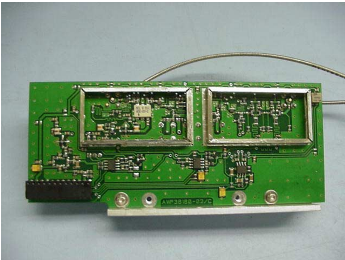
TX IF Board, Top Side
