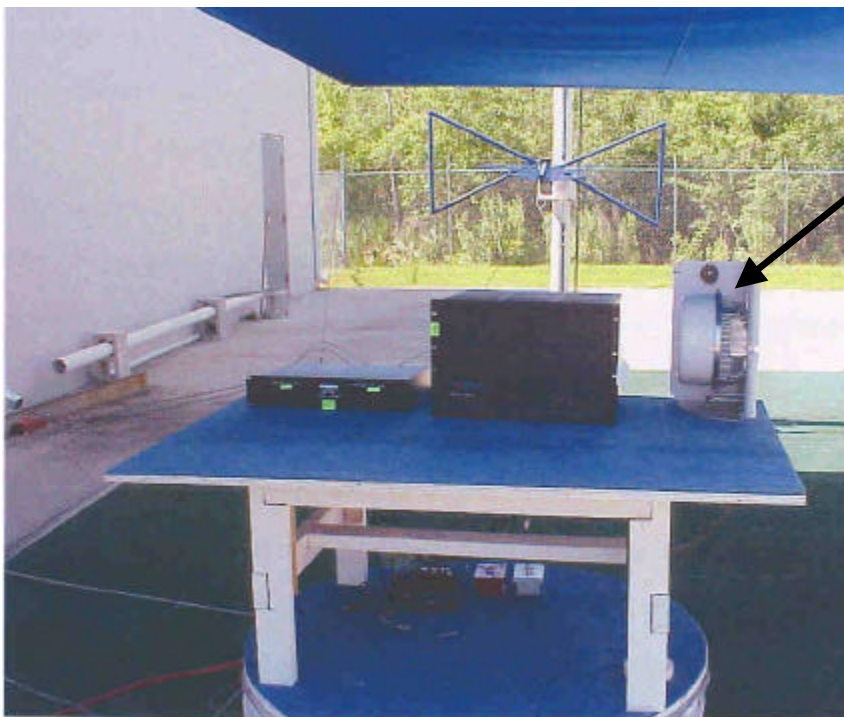
Sector ODU and Antenna
