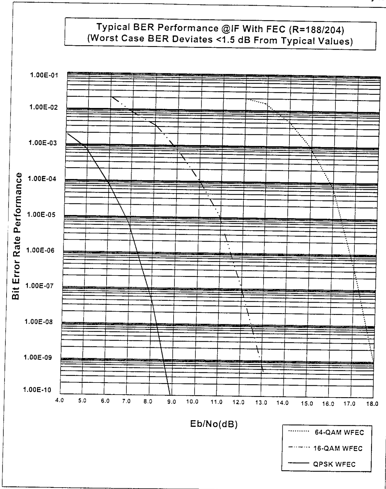
Figure 6-1 – Bit Error Rate Performance
