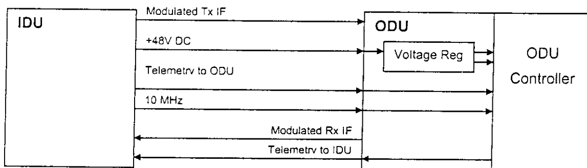
Figure 3-12 – Signal Distribution in the IDU/ODU System
