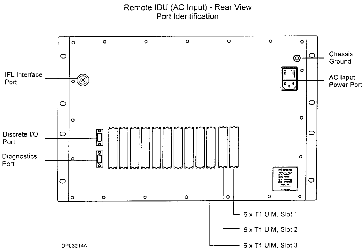
Figure 8-1 – Remote Terminal IDU (AC Input) Rear View
