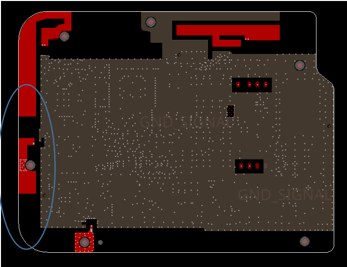
Figure 1. B015 PCB Antenna PCB-63693-003
