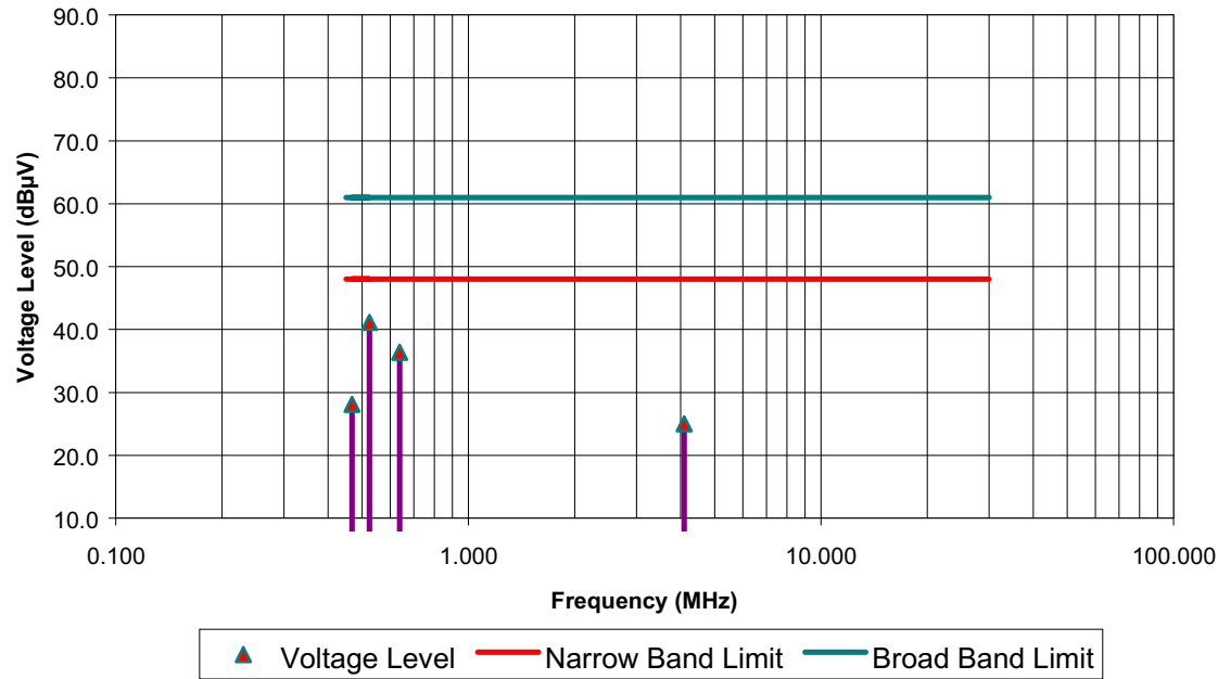
AC Conducted Emissions - Line #2 (Neutral) RIM BlackBerry Wireless Handheld, Model R1900G-1-4 Test Configuration #1: BlackBerry Wireless Handheld with PWR-02908-003 AC Charging Adapter
