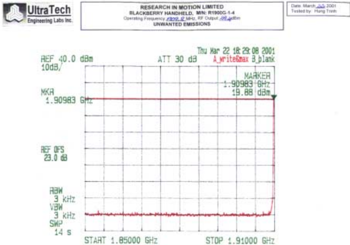
Plot 19: Conducted Spurious Emissions Transmitter Frequency: 1909.8 MHz
