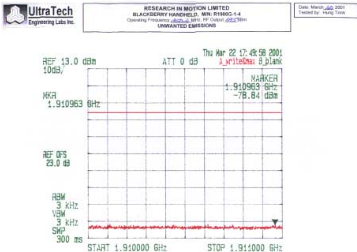
Plot 10: Conducted Spurious Emissions Transmitter Frequency: 1850.2 MHz
