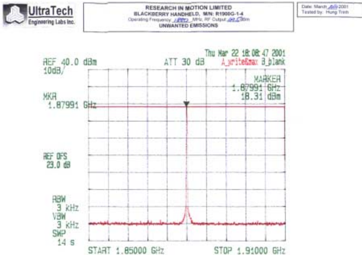
Plot 14: Conducted Spurious Emissions Transmitter Frequency: 1880.0 MHz
