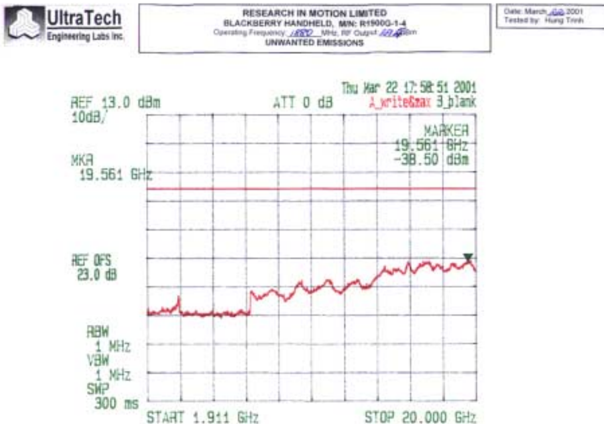
Plot 16: Conducted Spurious Emissions Transmitter Frequency: 1880.0 MHz
