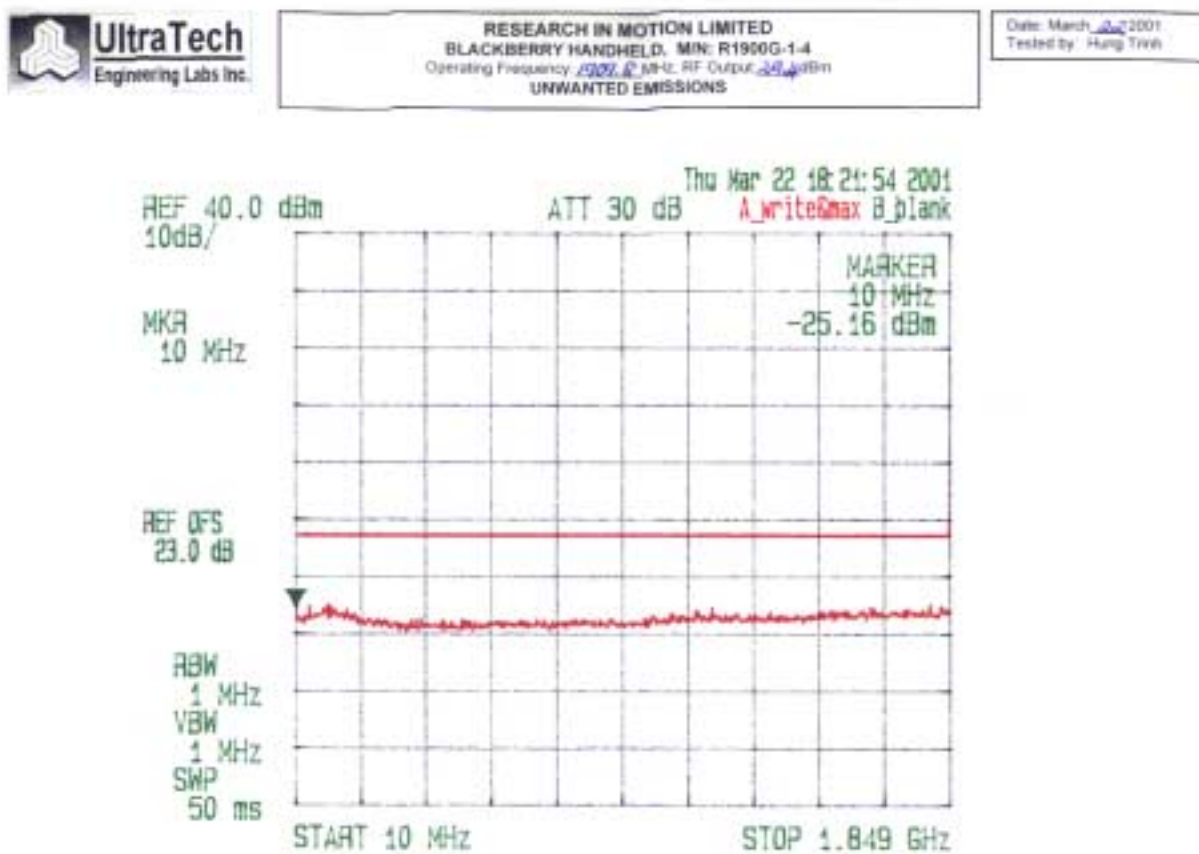
Plot 17: Conducted Spurious Emissions Transmitter Frequency: 1909.8 MHz
