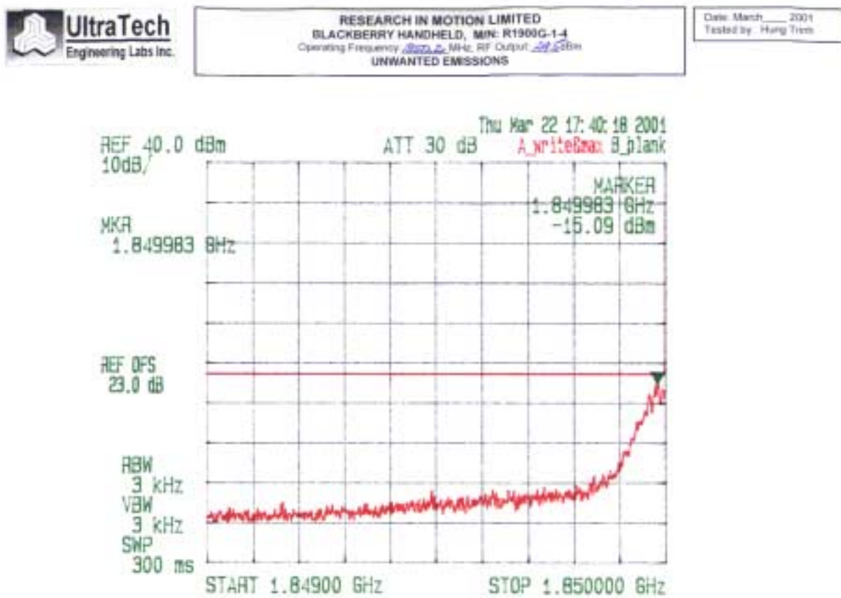
Plot 8: Conducted Spurious Emissions Transmitter Frequency: 1850.2 MHz
