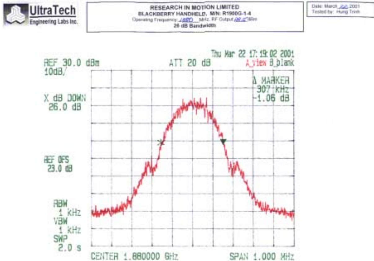
Plot 5: -26dBc Bandwidth Transmitter Frequency: 1880.0 MHz
