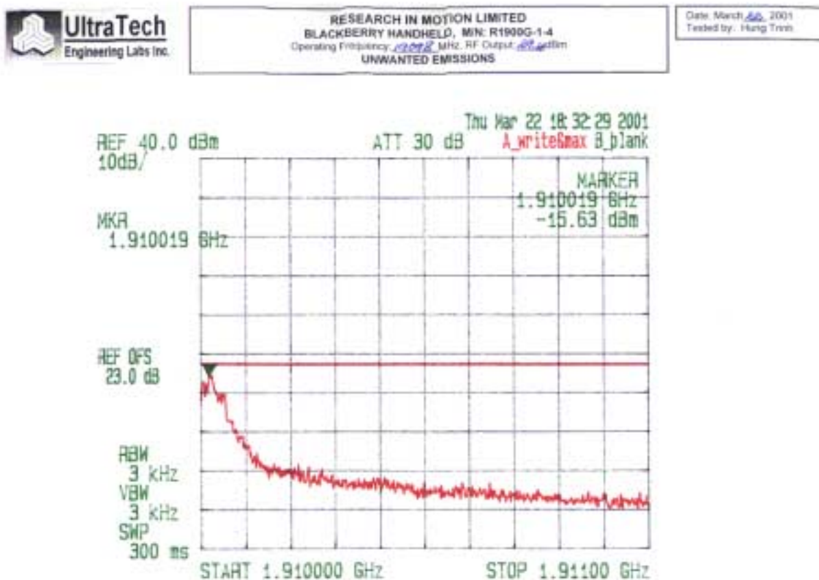
Plot 20: Conducted Spurious Emissions Transmitter Frequency: 1909.8 MHz
