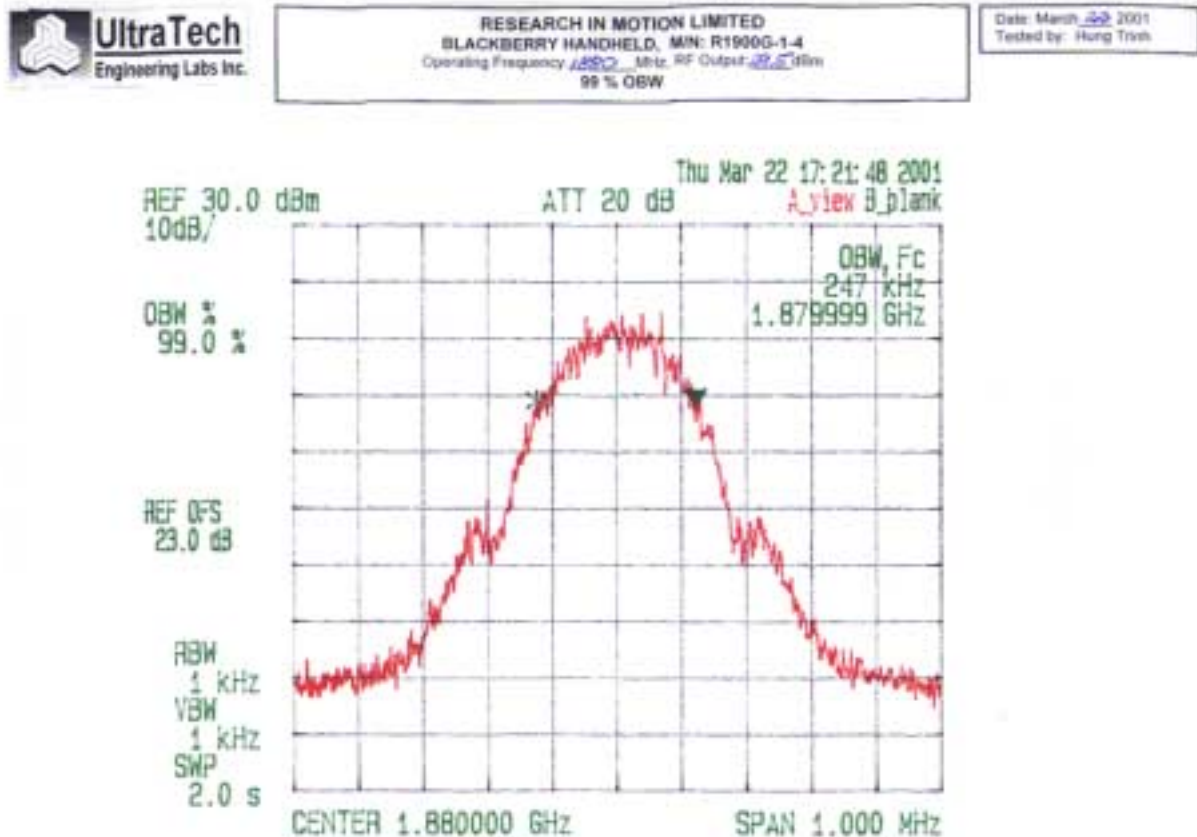
Plot 2: 99% Occupied Bandwidth Transmitter Frequency: 1880.0 MHz
