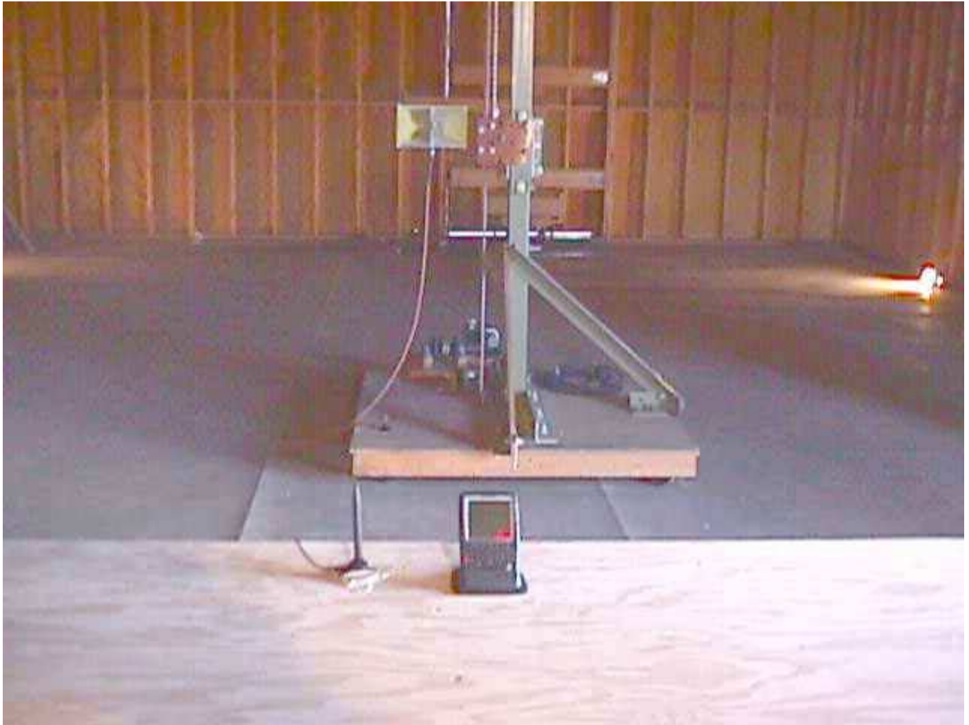
Test Configuration # 5: EUT In Cradle
