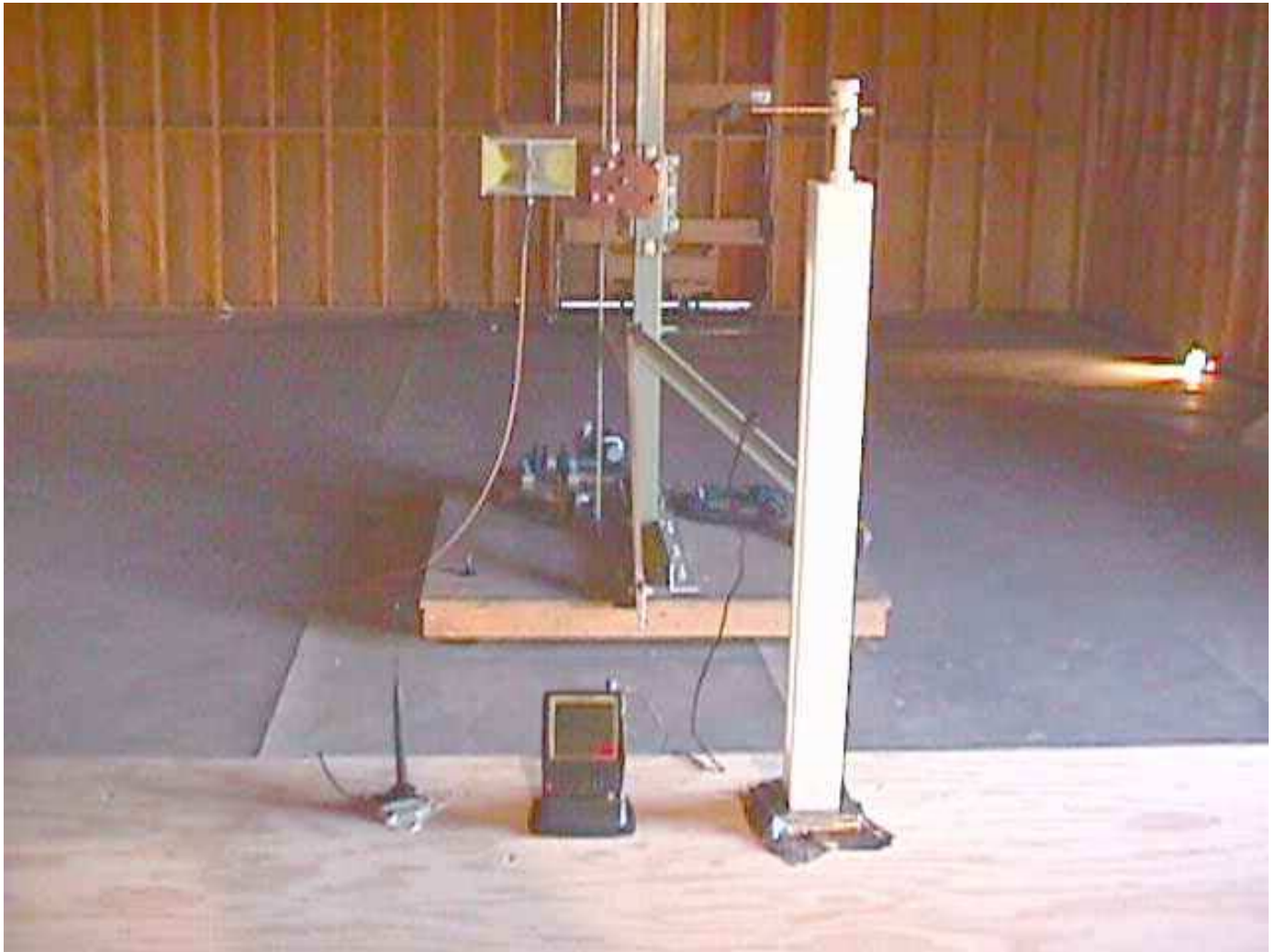
Test Configuration # 1: EUT in Cradle with Headset
