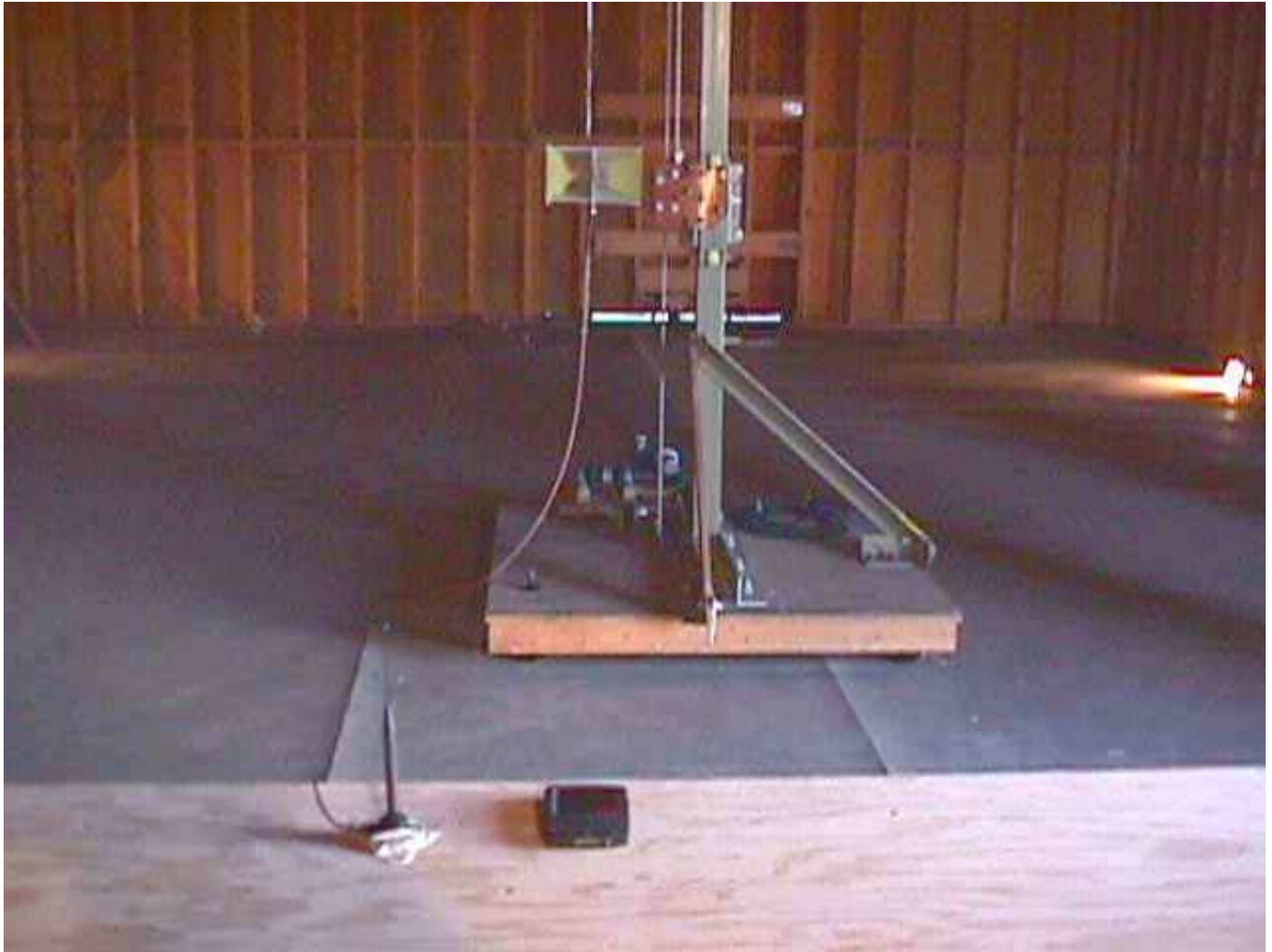
Test Configuration # 3: EUT Standalone (Laid Flat)
