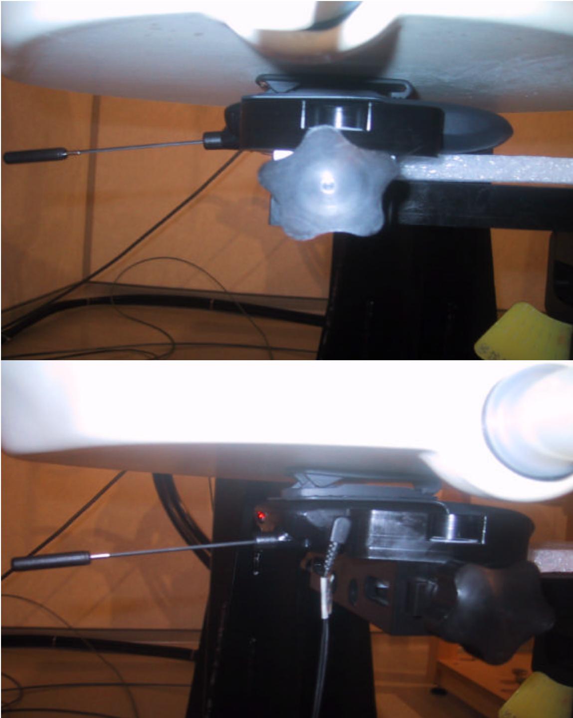
Figure E6. Body worn configuration extended antenna with holster and headset
