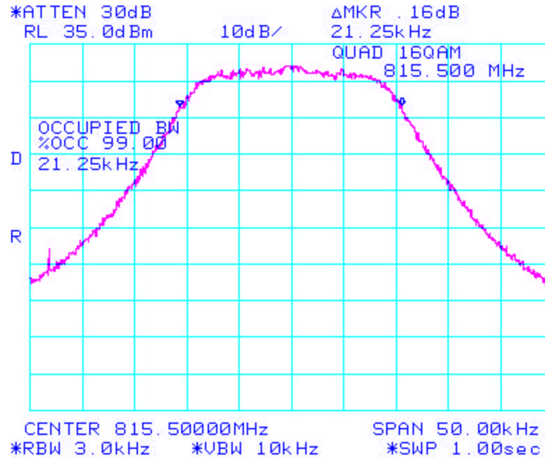
Figure 23: Occupied Bandwidth (99%)
