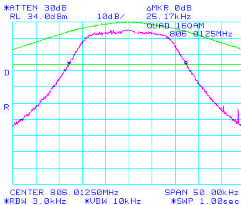
Figure 30: -26 dBc Bandwidth
