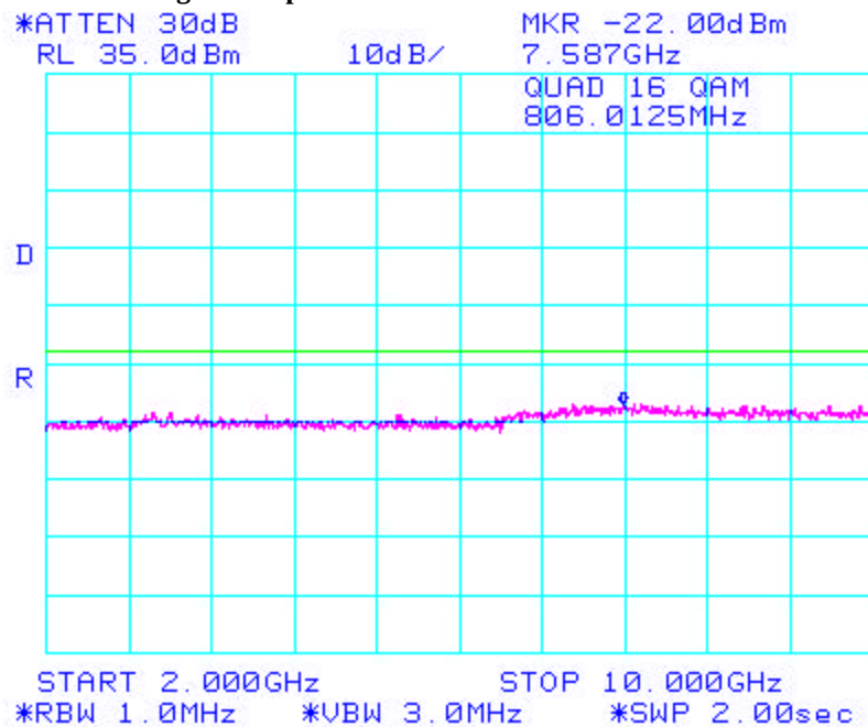
Figure 8: Spurious Conducted Emissions 2.1051
