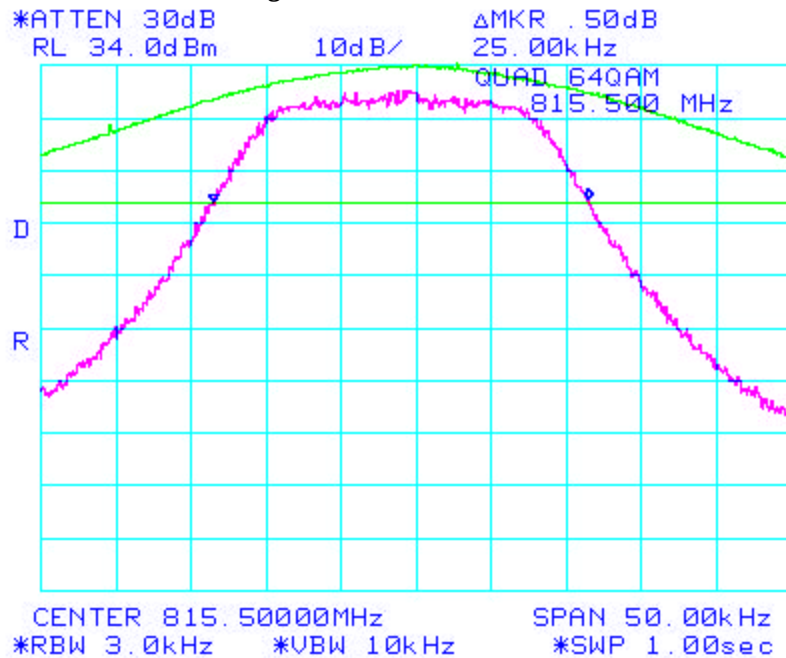
Figure 34: -26 dBc Bandwidth
