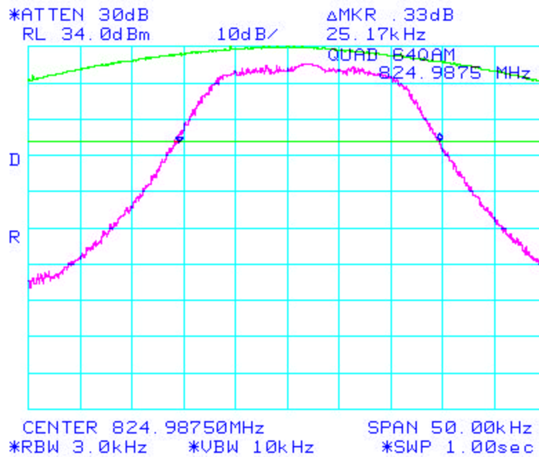
Figure 35: -26 dBc Bandwidth
