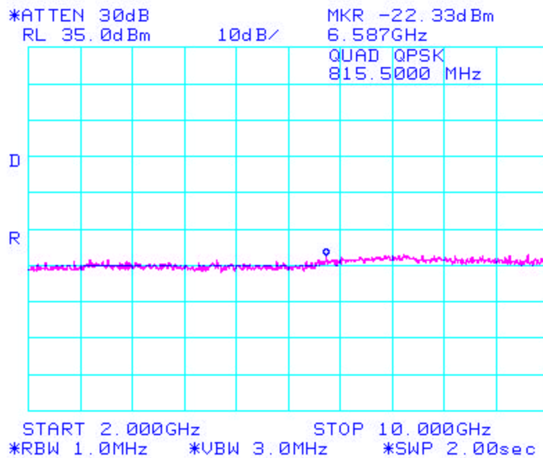
Figure 4: Spurious Conducted Emissions 2.1051
