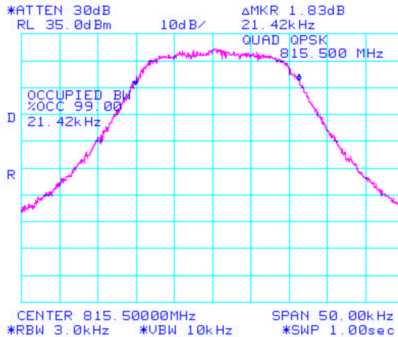
Figure 20: Occupied Bandwidth (99%)
