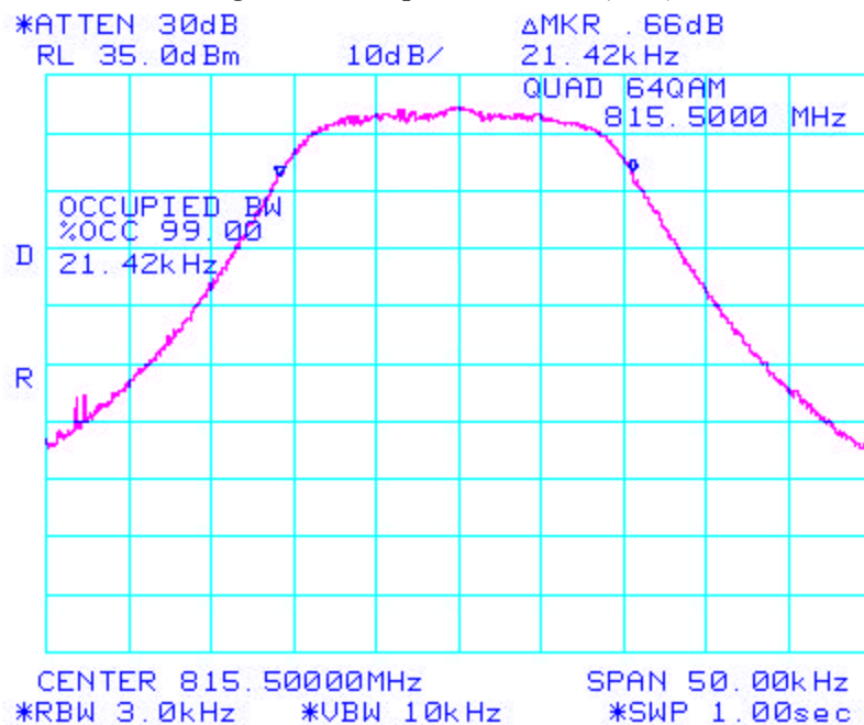
Figure 26: Occupied Bandwidth (99%)
