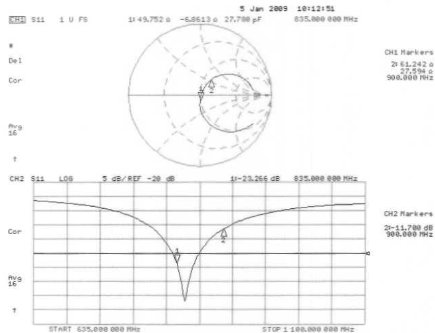
Impedance Measurement Plot for Head TSL
