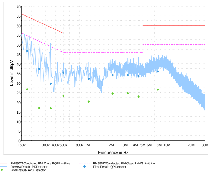
Figure 1-6: N Lines
