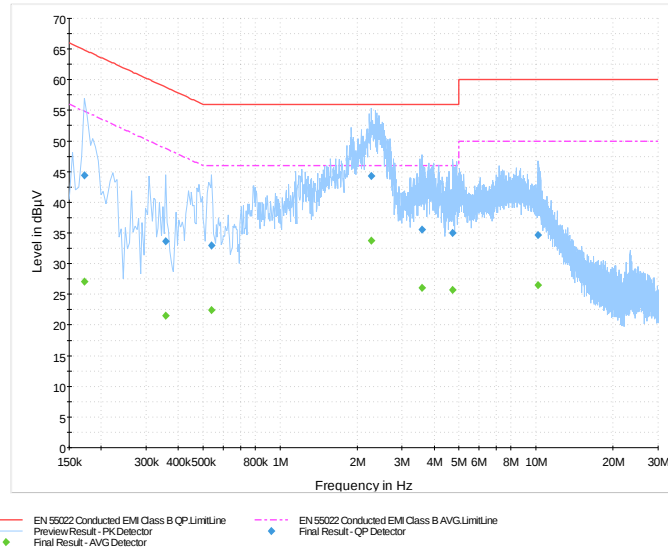
Figure 1-11: L1 lines
