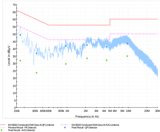
Figure 1-5: L1 lines
