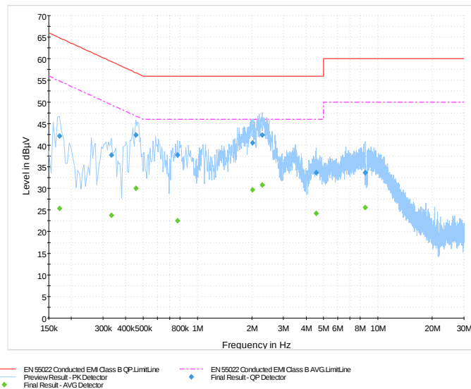
Figure 1-12: N Lines
