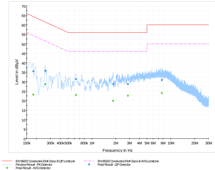
Figure 1-2: N Lines
