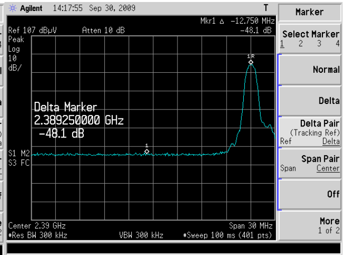
Figure 2-8: Band-Edge Compliance of RF Rad. Emissions.
