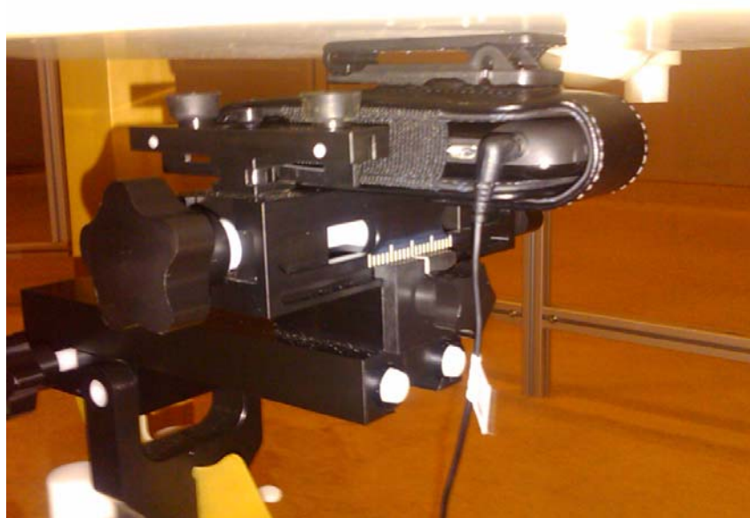
Figure E7. Body-worn configuration (Vertical Holster, headset 1, back facing phantom)
