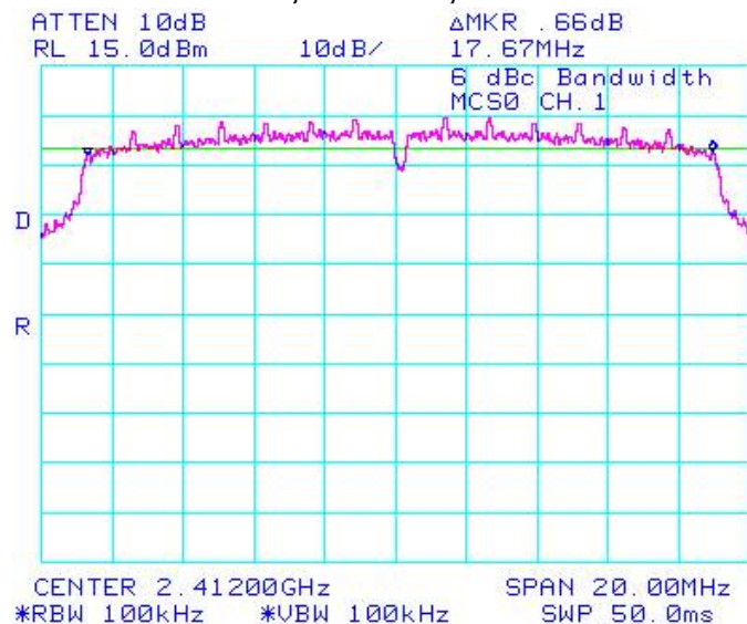
Figure 4-7: 6 dB Bandwidth
