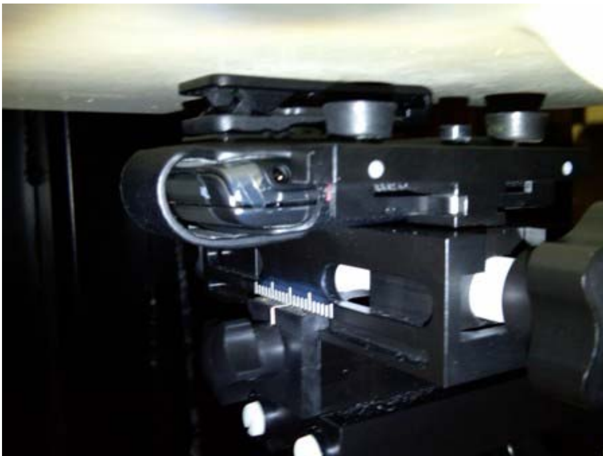
Figure E8. Body-worn configuration (Vertical Holster, back facing phantom)
