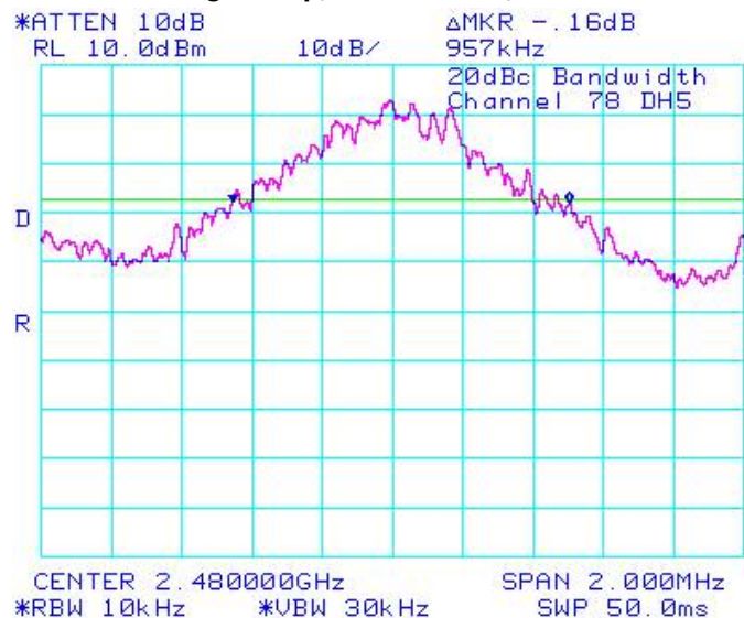
Figure 3-3: 20 dB Bandwidth
