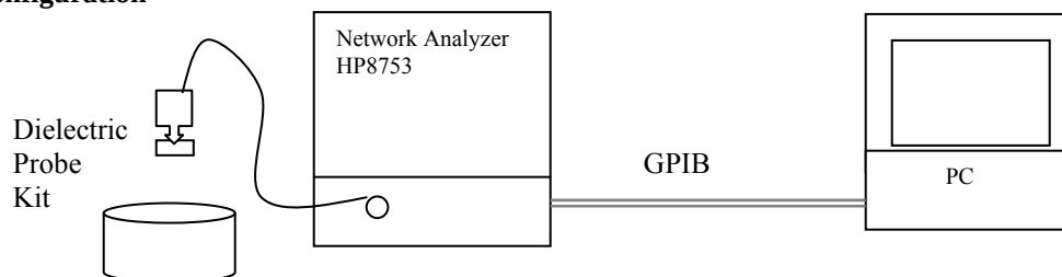
Figure 6.2.1 Test configuration
