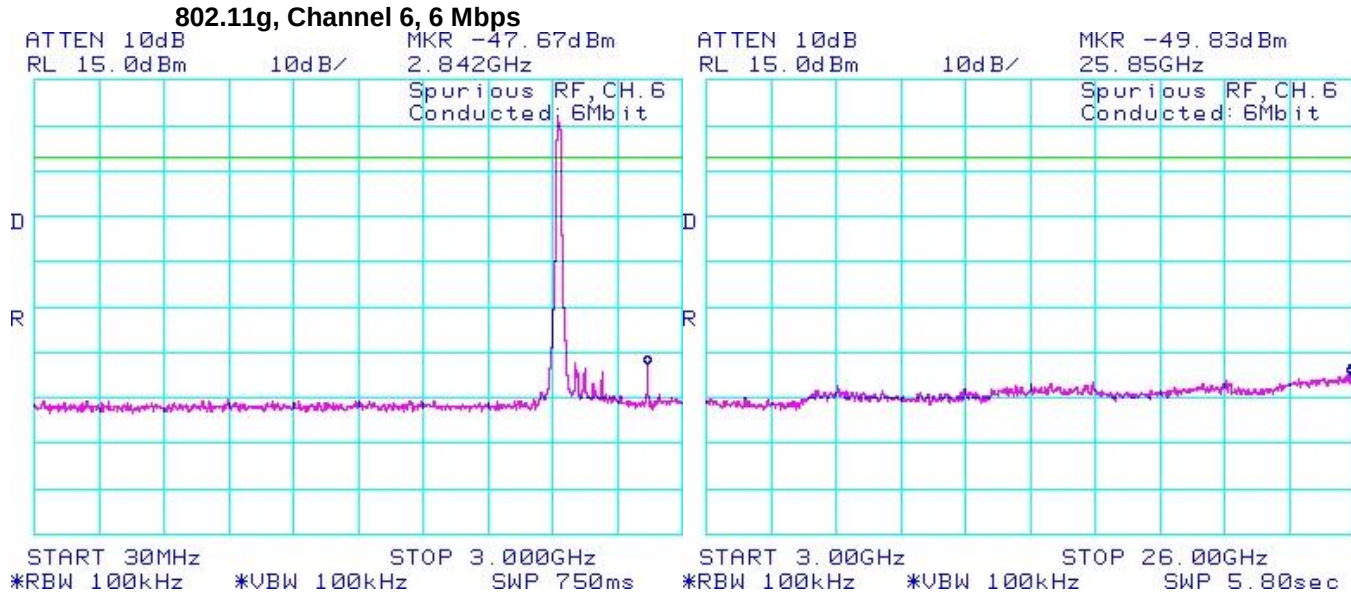
Figure 4-29: Spurious Conducted RF Emissions
