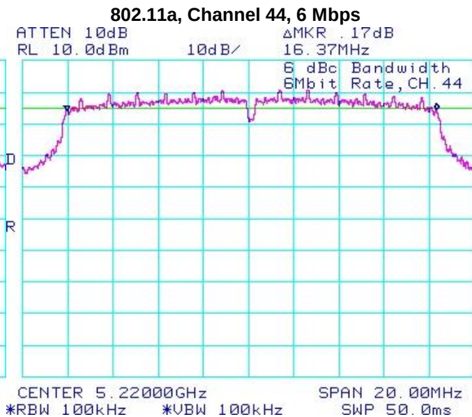
Figure 5-2: 6 dB Bandwidth
