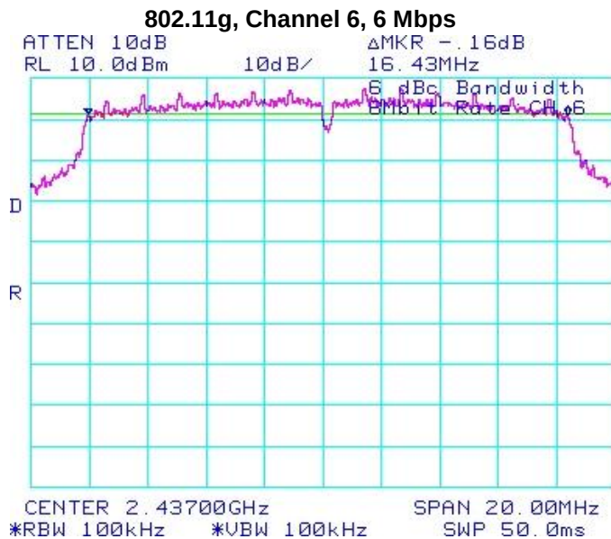
Figure 4-5: 6 dB Bandwidth
