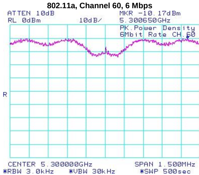
Figure 5-20: Peak Power Spectral Density
