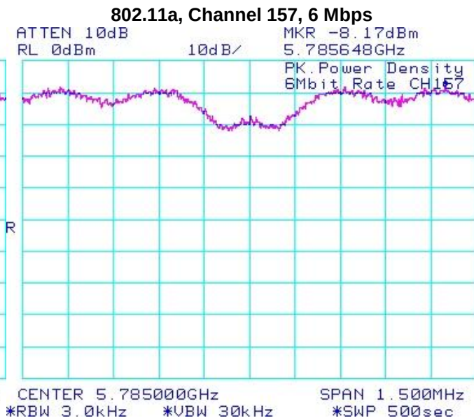
Figure 5-23: Peak Power Spectral Density
