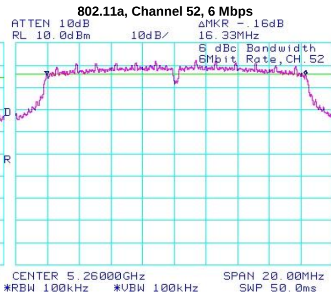
Figure 5-4: 6 dB Bandwidth
