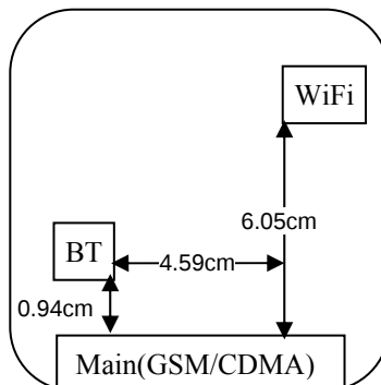
Figure 1.9.1. RDR61CW Back view of device showing closest distance between antenna pairs
