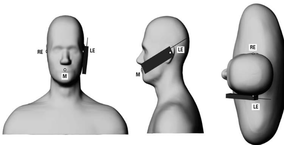
Figure 8.2.2. Phone position 1, “cheek” or “touch” position. The reference points for the right ear (RE), left ear (LE) and mouth (M), which define the reference plane for phone positioning, are indicated. The shoulders are shown for illustration purposes only.
