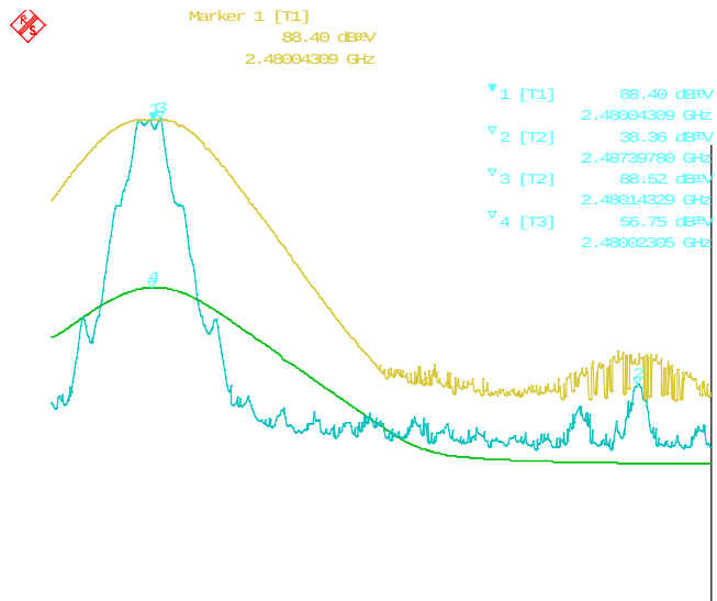
Figure 2-4: Band-Edge Compliance of RF Rad. Emissions Bluetooth, Single freq., Static PBRS, DH5, Channel 78, Pol: H, Detector: PK
