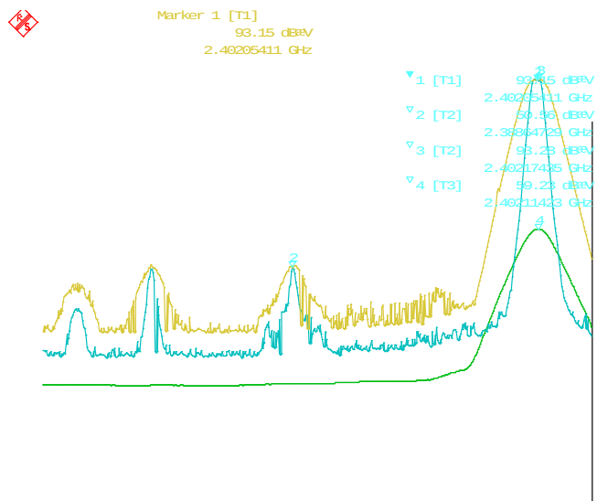
Figure 2-2: Band-Edge Compliance of RF Rad. Emissions. Bluetooth, Single freq., Static PBRS, DH5, Channel 0, Pol: H, Detector: PK
